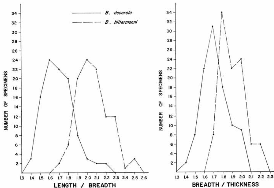
TEXT-FIG. 6. Diagrams showing comparison of length/breadth and breadth/thickness ratios of 100 specimens of Bolivinoidea decorata (Jones) and 100 specimens of B. hiltermanni sp. nov. All specimens of B. decorata are from sample C10, Belemnitella mucronata Zone, Culver Cliff. All specimens of B. hiltermanni are from sample C29, Actinocamax quadratus Zone, Culver Cliff.
