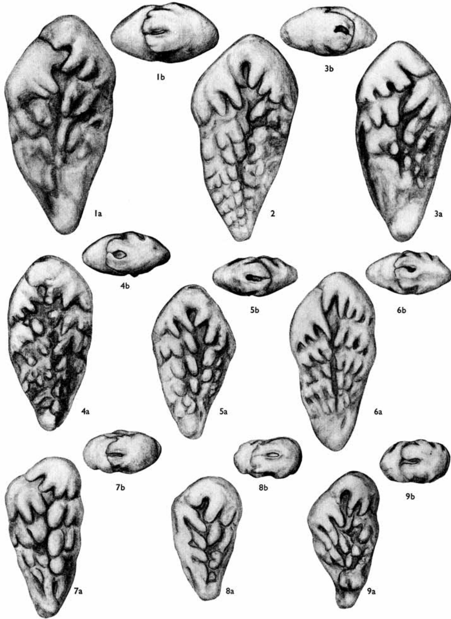
BARR, Upper Cretaceous Bolivinooides
