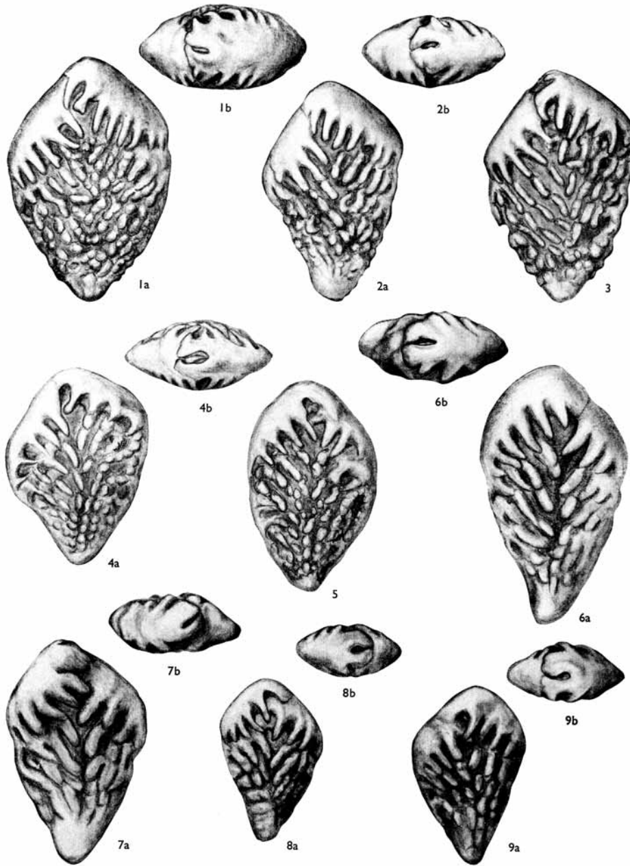
BARR, Upper Cretaceous Bolivinoides
