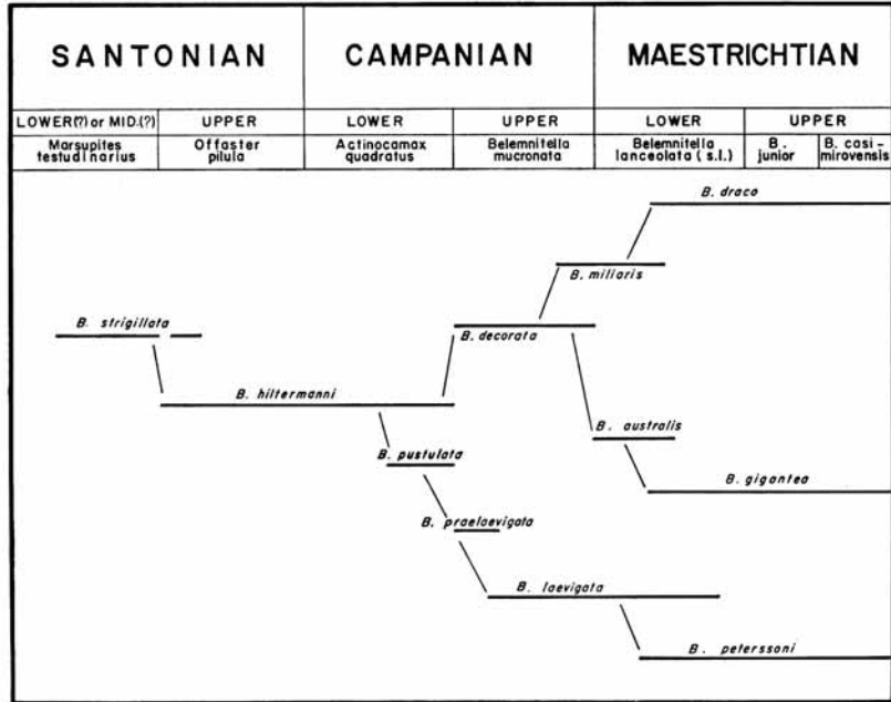
TEXT-FIG. 5. Diagram showing the stratigraphic ranges and suggested phylogeny of various species of Bolivinoidea .
