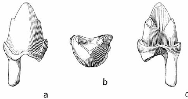
TEXT-FIG. 9. Cf. Spalacotherium tricuspidens Owen, left lower molar, M21103, \times 30 . a, Labial view; b, occlusal view; c, lingual view.
