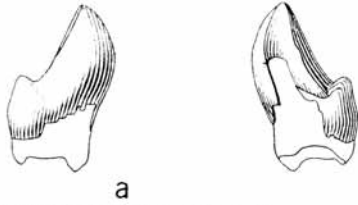
TEXT-FIG. 5. Loxaulax valdensis Simpson, probably an upper incisor, M21100, \times 7.5 . a and b , Lateral views.
