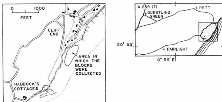
TEXT-FIG. 1. Cliff End Bone Bed, locality map. Area depicted in map on left shaded in the index map on right.
