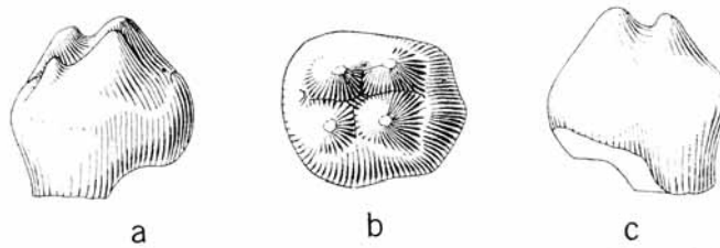
TEXT-FIG. 4. Loxaulax valdensis Simpson, anterior upper premolar, probably a right premolar, M21106, \times 30 . a , Labial view; b , occlusal view; c , lingual view.
