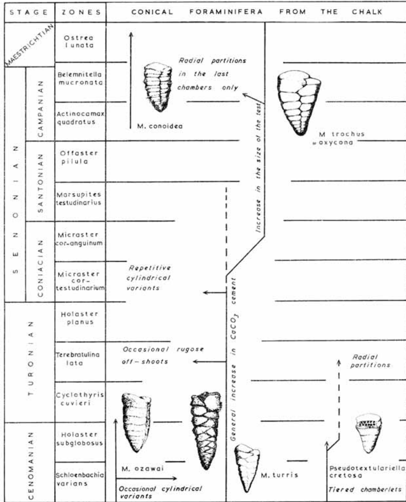
TEXT-FIG. 5. Diagram showing the ranges and development of some conical foraminifera from the Chalk (Upper Cretaceous).
