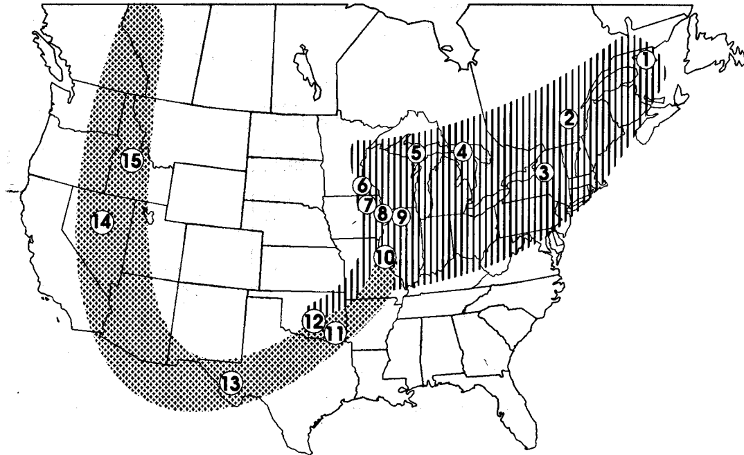
TEXT-FIG. 7. Distribution of late Ordovician graptolite biofacies in United States and adjacent parts of Canada. Vertical ruling and stippling represent the Laurentian Biofacies and the Oceanic Biofacies, respectively. Numbered localities and areas are as follows: 1, Anticosti Island, Quebec; 2, Saint Lawrence Lowlands, Quebec; 3, Mohawk and Black River valleys, New York State; 4, Manitoulin Island, Ontario; 5, Upper Peninsula of Michigan; 6, Rifle Hill Quarry, southern Minnesota; 7, Postville, Iowa; 8, Graf, Iowa; 9, north-western Illinois; 10, Saint Louis region, Missouri; 11, Ouachita Mountains, eastern Oklahoma; 12, Arbuckle Mountains, Oklahoma; 13, Marathon region, west Texas; 14, central Nevada; 15, Trail Creek, Idaho. Note that the two biofacies overlap in the Arbuckle Mountains. Map adapted from Finney (1986) and Goldman and Bergström (1995).
