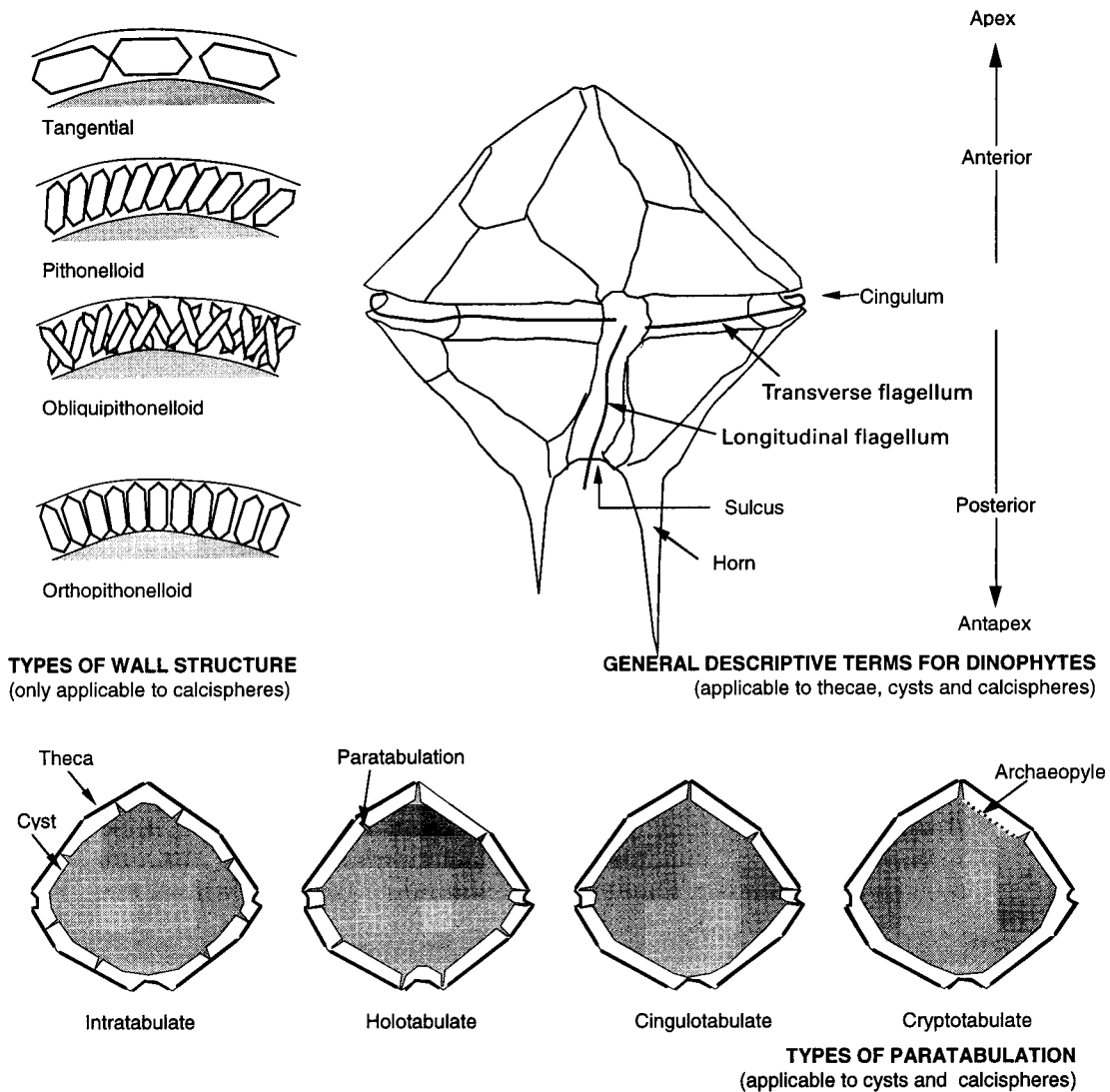
TEXT-FIG. 15. Terms used in the description of calcispheres. N.B. Calcispheres are formed by dinoflagellates and their terminology is independent of that used for other calcareous nannoplankton.
