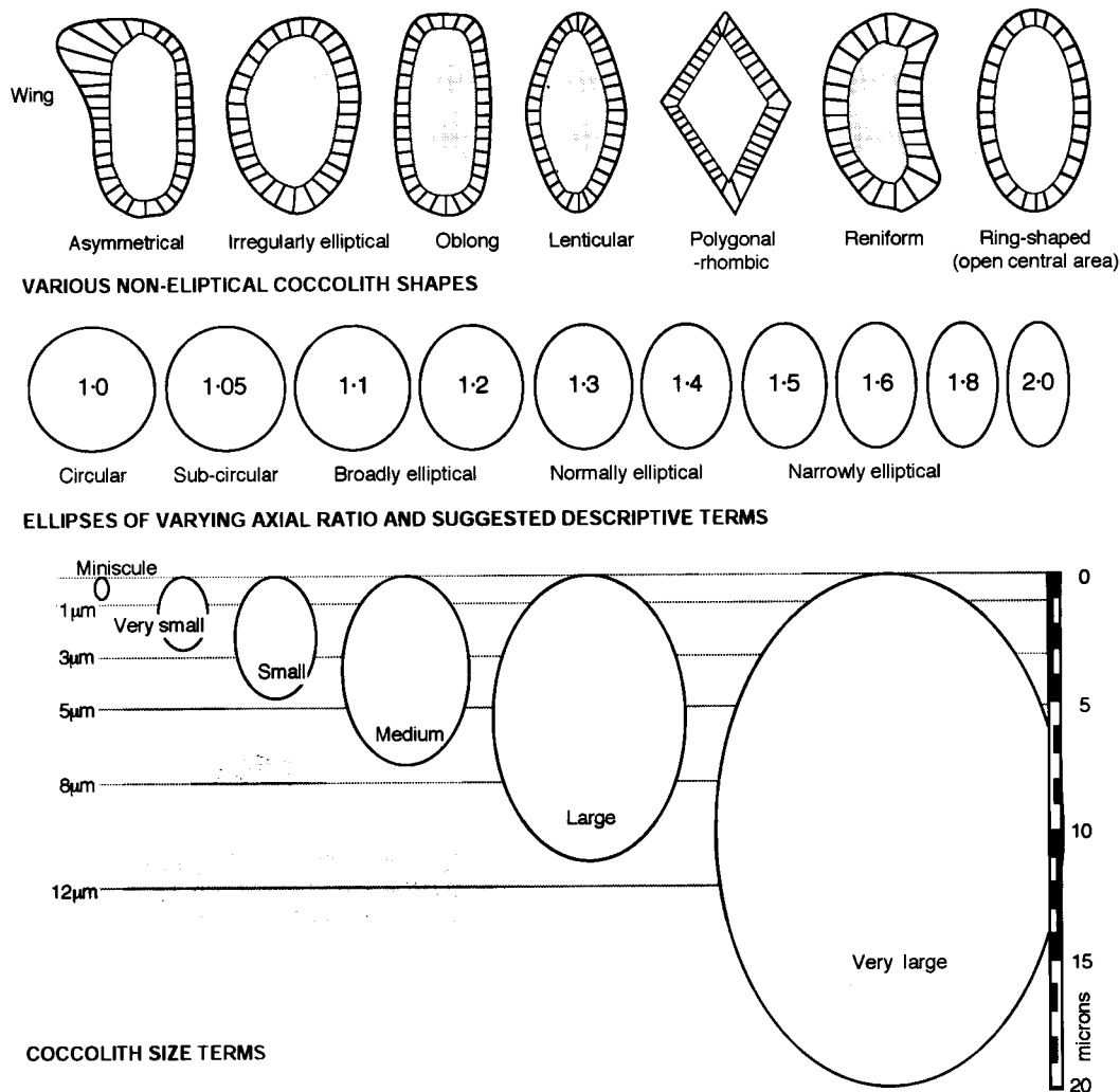
TEXT-FIG. 3. Coccolith sizes and shapes.
