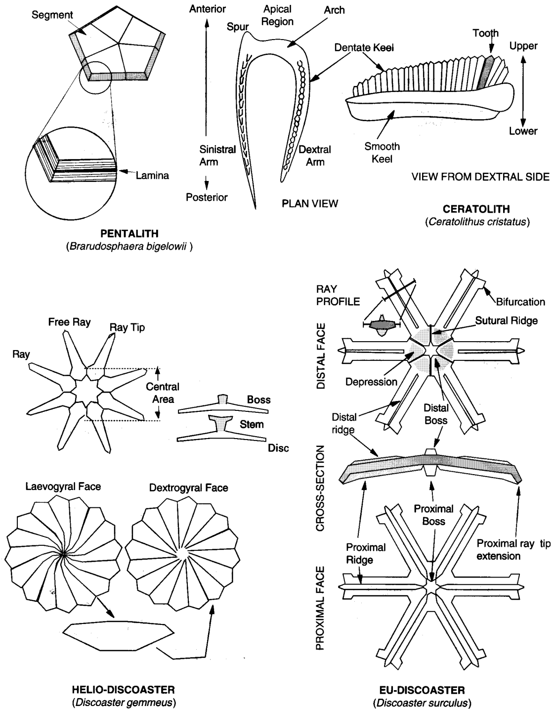
TEXT-FIG. 11. Special terms applied to Braarudosphaeraceae, Ceratolithaceae and Discoasteraceae. N.B. The terms applied to the description of heterococcoliths may also, where appropriate, be applied to these groups, and vice versa.
