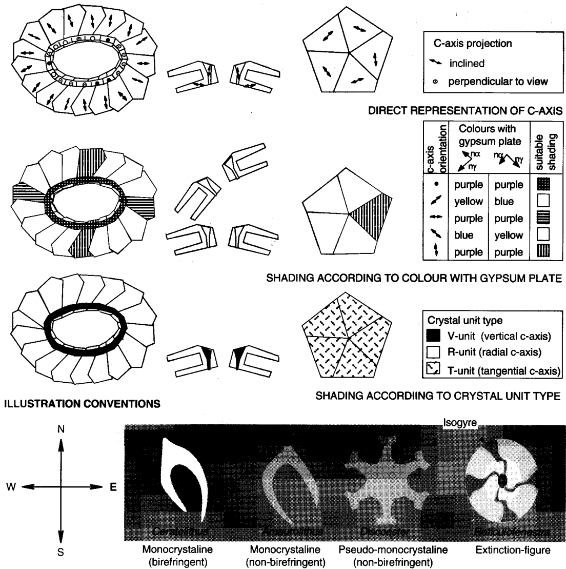
TEXT-FIG. 8. Crystallography: the diagrams showing illustration conventions are based on Watznaueria (plan and side views) and Braarudosphaera ; the figures in the dark box represent the appearance of nannofossils in the light microscope, with cross-polarized light.
