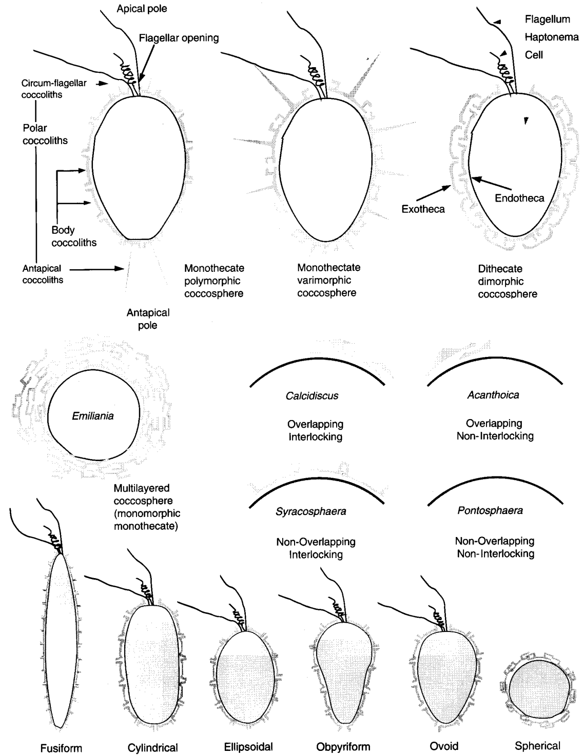
TEXT-FIG. 1. Coccosphere related terms.
