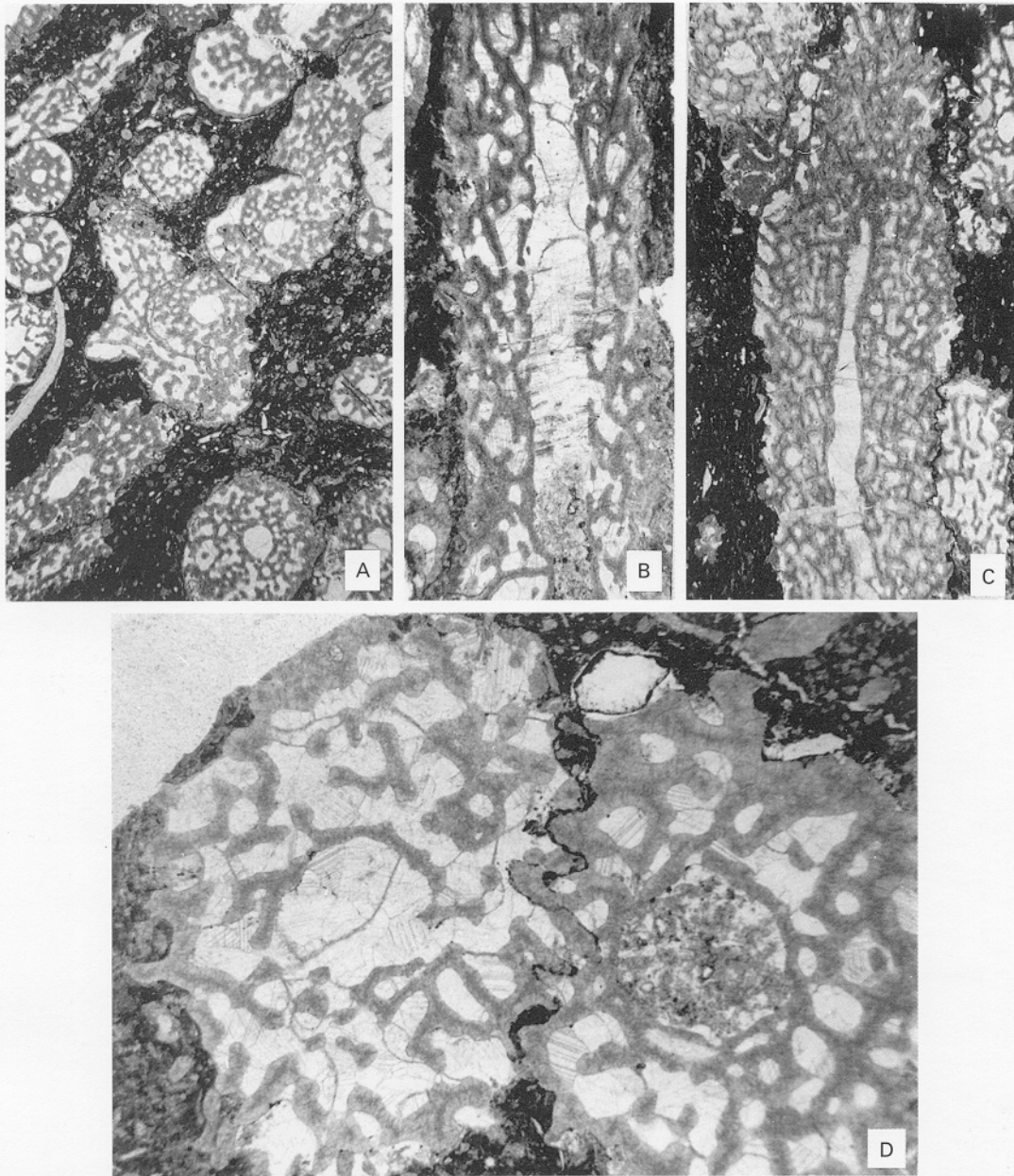
TEXT-FIG. 8. A, Amphipora ramosa (Philips 1841)?; specimen from core (McGill Redpath Museum RM 20-5341), Swan Hills field, north central Alberta at 8901 ft [10-34-63-11W5th mer]. Note the outgrowth on the central stem that could be a root structure and the great variation in axial canals and peripheral membranes in a single slide; \times 5 . B-D, Amphipora ramosa (Phillips, 1841). B, neoparatype PO 309.B3; axial section, showing wide axial canal with many pores, well-developed pillars, and a poorly developed peripheral membrane on the middle left; \times 10 . C, neotype suite PO 308.A15; axial section, showing discontinuous membrane, well developed in the upper right and largely absent below on this side, well-developed pillars holding the membrane, and tabulae crossing the axial canal; \times 5 . D, section PO 308.A9; cross sections from the neotype suite, showing fibrous microstructure, post-and-bridge construction, dissepiments and tabulae; internal spaces largely open in the stem on the left and closed on that on the right; \times 20 .
