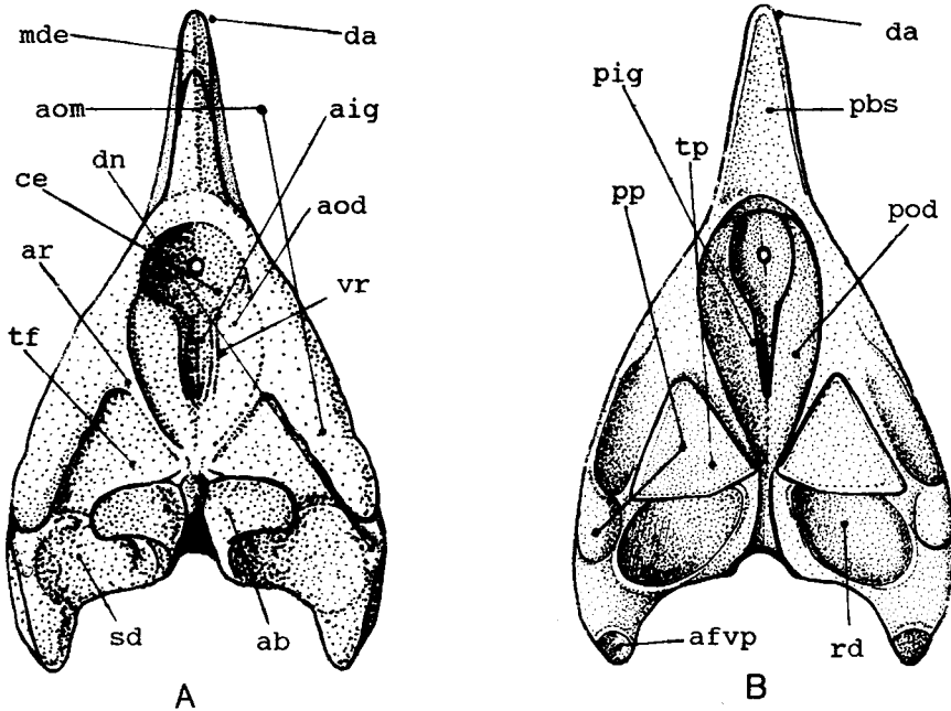
TEXT-FIG. 18. Placocystella africana (Reed, 1925). Reconstruction of a tail ossicle. A, anterior view; B, posterior view. Abbreviations as in the text.
