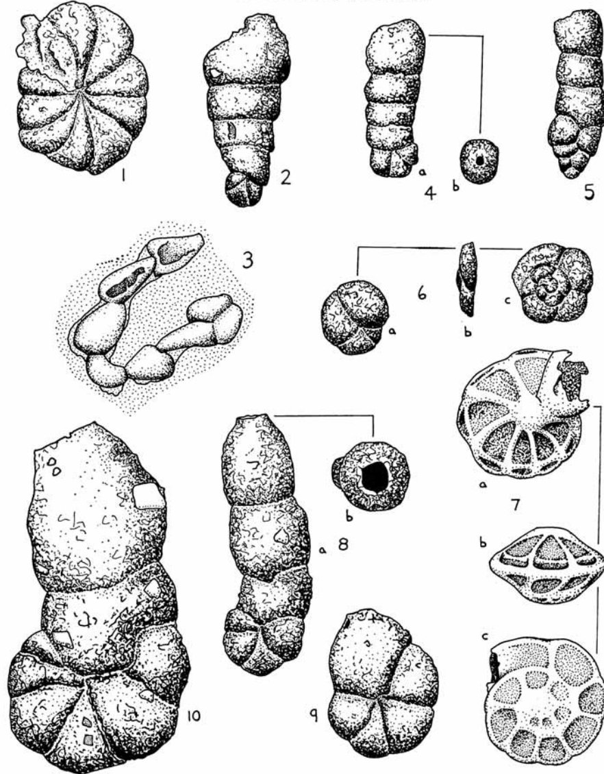
TEXT-FIG. 1. (1) Cribrostomoides canui (Cushman). Mepal. \times 60 . (2) Ammobaculites cf. reophaciformis Cushman. Mepal. \times 60 . (3) Bullopora rostrata Quenstedt. Knapwell. \times 60 . (4)a, b. Ammobaculites agglutinans (d'Orbigny). Mepal. \times 75 . (5) Bigenerina cf. nodosaria d'Orbigny. Mepal. \times 75 . (6)a-c. Trochammina squamata Jones and Parker. Mepal. \times 75 . (7)a-c. Voorthuysenia tenuicostata (Bartenstein and Brand). Mepal. \times 75 . (8)a, b. Ammobaculites coprolithiformis (Schwager). Mepal. \times 40 . (9), (10) Ammobaculites coprolithiformis (Schwager). Knapwell. \times 40 .
