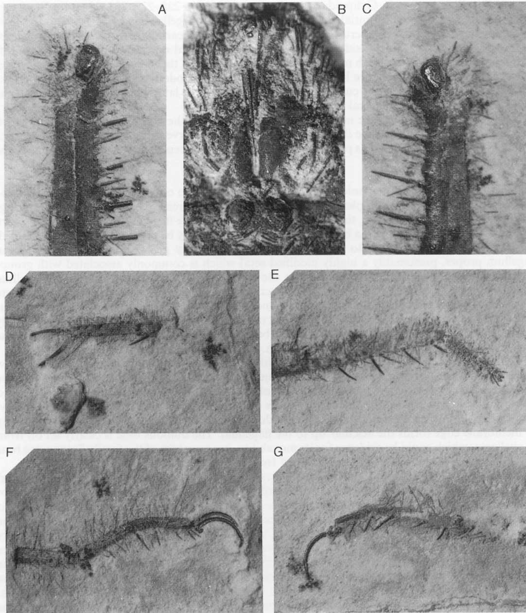
TEXT-FIG. 6. Cratosolpuga wunderlichi Selden, gen. et sp. nov. Holotype; Cretaceous (Aptian), Crato Formation; Ceará Province, Brazil; Sol 1. A, C, distal tibia and tarsus of pedipalp. A, left \times 20 ; C, right \times 23 . B, anterior carapace margin with eyes, and basal chelicerae showing male flagella; basal section of whip of left flagellum is missing; whips disappear into matrix between cheliceral bases; \times 23 . D-G, tarsi of legs left III, right III, left IV and right IV, respectively; showing basitarsal spines (leg III), hairs and trichobothria, and telotarsal claws (missing from right III) with distal joint; \times 15 .
