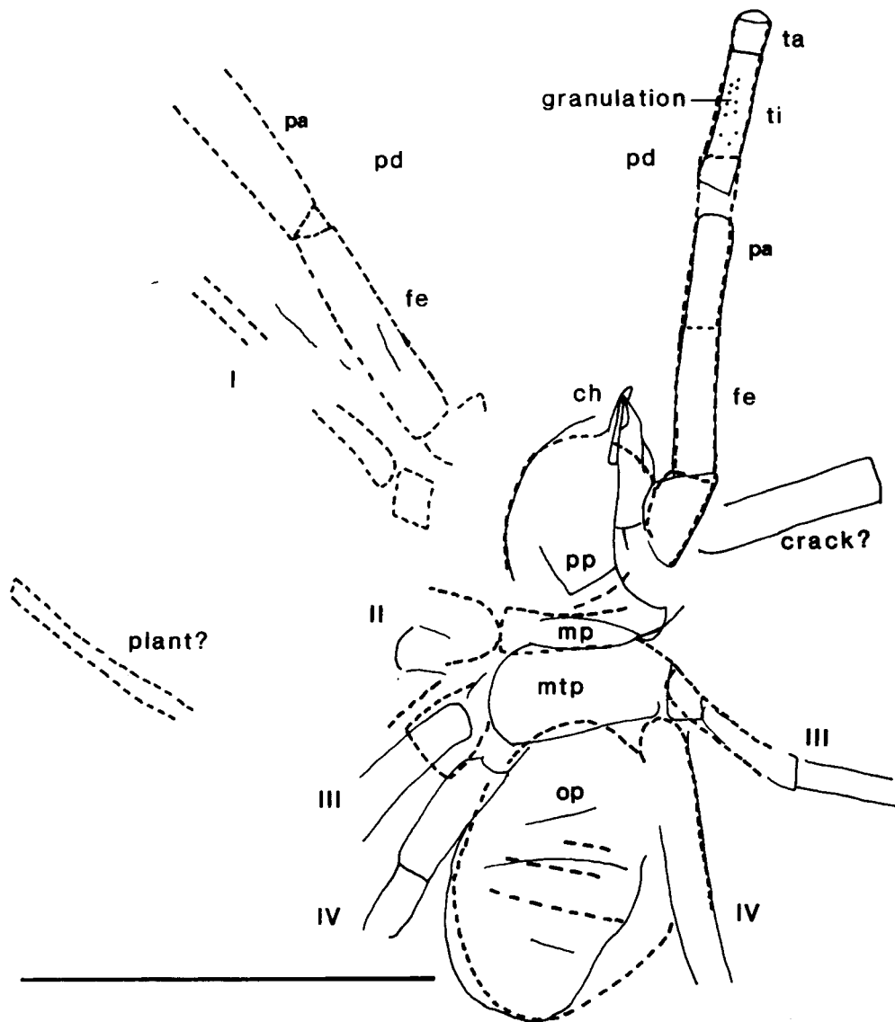
TEXT-FIG. 2. Composite camera lucida drawing of Protosolpuga carbonaria Petrunkevitch, 1913. Holotype, Peabody Museum 00155/B1336; Upper Carboniferous (Westphalian D), Francis Creek Shale; Mazon Creek, Illinois. Solid lines, ventral side; dashed lines, dorsal side. Scale bar represents 10 mm.
