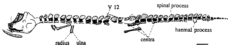
TEXT-FIG. 9. NMP ČM 1462 (Pb 26, 27). Miocene; Lužice near Břilina (north Bohemia, Czech Republic). Skeleton in lateral aspect, preserved in silicified diatomites. Scale bar represents 2 mm.
