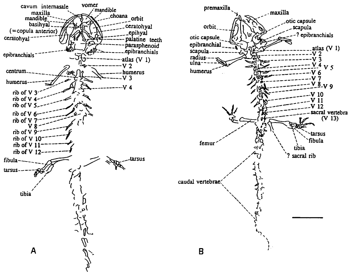
TEXT-FIG. 6. Brachycormus noachicus (Goldfuss, 1831), A, MB Am.928.1–2, holotype of Oligosemia gerhardi Herre, 1949; skeleton in ventral view. B, MB Am.930.1, holotype of Tylototriton kosswigi Herre, 1949; skeleton in dorsal view. Scale bar represents 5 mm.
