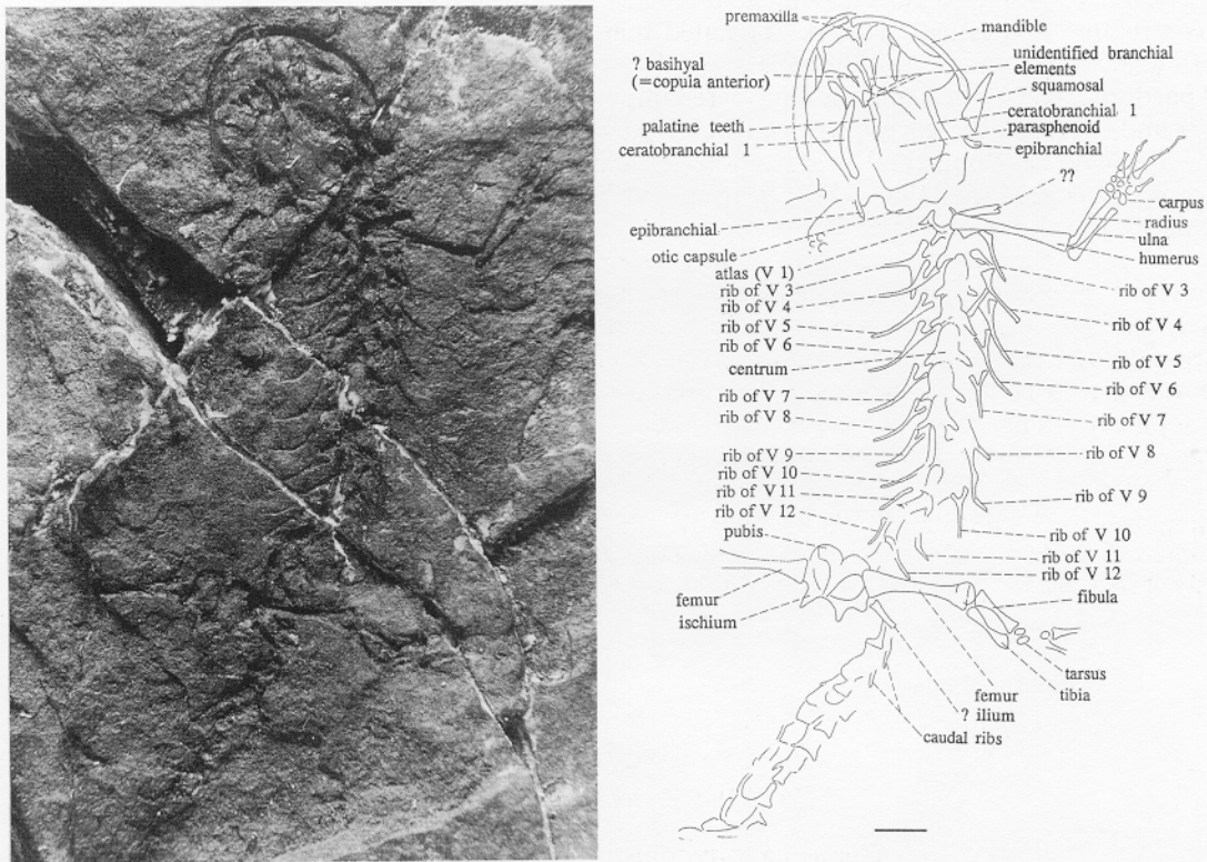
TEXT-FIG. 1. Brachycormus noachicus (Goldfuss, 1831). PIUB Ro 4429, holotype; (formerly Goldfuss 1307 A); Upper Oligocene; Orsberg. Scale bar represents 2 mm.
