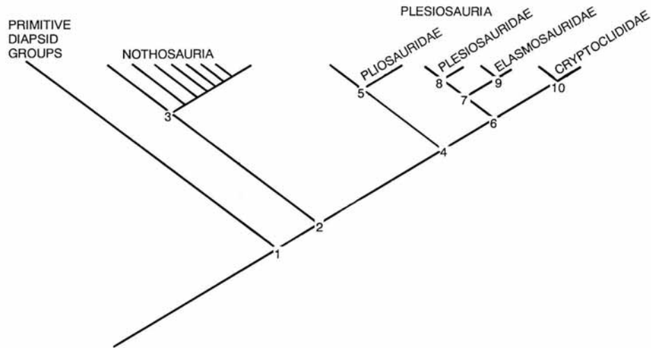
TEXT-FIG. 7. Phylogenetic analysis showing interrelationships of major sauropterygian groups, based on characters of the cheek and orbit. Numbered nodes 1 to 10 are characterized in the text.
