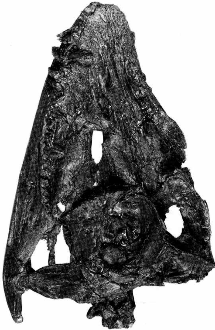
TEXT-FIG. 1. Cryptoclidus eurymerus (Phillips). PETMG R.283.412; dorsal view of skull; Dogsthorpe, near Peterborough, UK; Lower Oxford Clay (Callovian); \times 0.5 .
