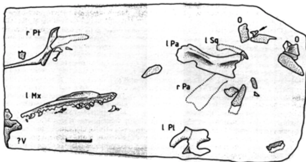
TEXT-FIG. 2. Parviraptor estesi gen. et sp. nov. BMNH 48388, holotype; Durliston Bay, Dorset; Purbeck Limestone Formation. Key: r, right; l, left; Mx, maxilla; O, osteoderm; Pa, parietal; Pl, palatine; Pt, pterygoid; Sq, squamosal; ?V, possible vertebral fragment. The arrow (top right) indicates the isolated archosaur tooth mentioned in the text. Scale bar represents 5 mm.
