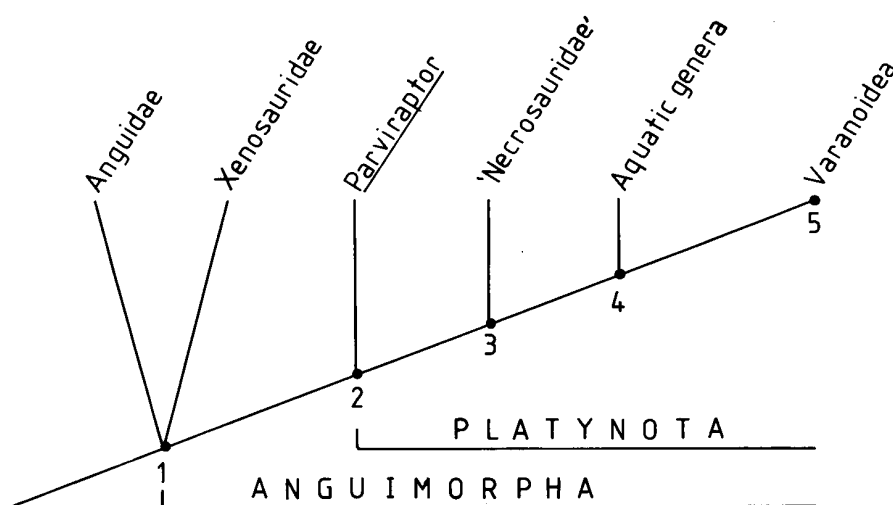
TEXT-FIG. 16. Cladogram showing hypothetical relationships for Parviraptor based on the work of Estes (1983), Borsuk-Bialynicka (1984) and Pregill et al. (1986). Key: Node 1, Anguimorpha (intramandibular septum; replacement teeth usually posterolingual; loss/reduction of subdental ridge; Meckel's groove opens anteroventrally; dorsal and cephalic osteoderms); Node 2, Platynota ( sensu Pregill et al. 1986) (well-developed subolfactory processes on frontals; teeth unicuspid, recurved, trenchant; reduction in maxillary/nasal contact; vomers narrow, more than twice palatine length; palatine as wide as it is long; osteoderms free of skull bones); Node 3, unnamed taxon (parietals fused; adductor muscles extend onto dorsal surface of parietal; splenial/dentary overlap reduced; vertebral condyle oblique [?R in aquatic genera] and waisted; postaxial cervical centra with fused hypapophyses bearing separate epiphyses); Node 4, unnamed taxon – aquatic genera denote aigialosaurs and mosasaurs (retracted nares; frontal trapezoid; maxilla does not underlie orbit; facial process of maxilla set posteriorly; plicidentine present [varies in 'necrosaurs']; reduced overlap of dentary and postdentary bones; separate epiphyses on cervical hypapophyses [varies in 'necrosaurs']; loss of caudal autotomy); Node 5, Varanoidea ( sensu Pregill et al. 1986, i.e. Varanidae, Lanthanotidae, Helodermatidae) (subolfactory processes of frontals usually meet in the midline; fewer than 13 maxillary teeth; supratemporal extends anterior to level of parietal notch).
