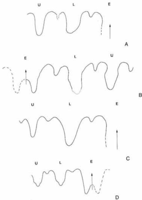
TEXT-FIG. 3. Leptoceratoid suture-lines. A, Karstenicerias beyrichoide sp. nov., fragmentary suture-line at H = 6 mm; BSM AS III 178. B, K. subtile (Uhlig), external suture-line of lectotype at H = 2.2 mm; GBAW 3949. C, K. hoheneggeri sp. nov., fragmentary suture-line at H = 3 mm; BSM AS III 179. D, K. hoheneggeri , external suture-line at H = 6 mm; BSM AS III 454.
