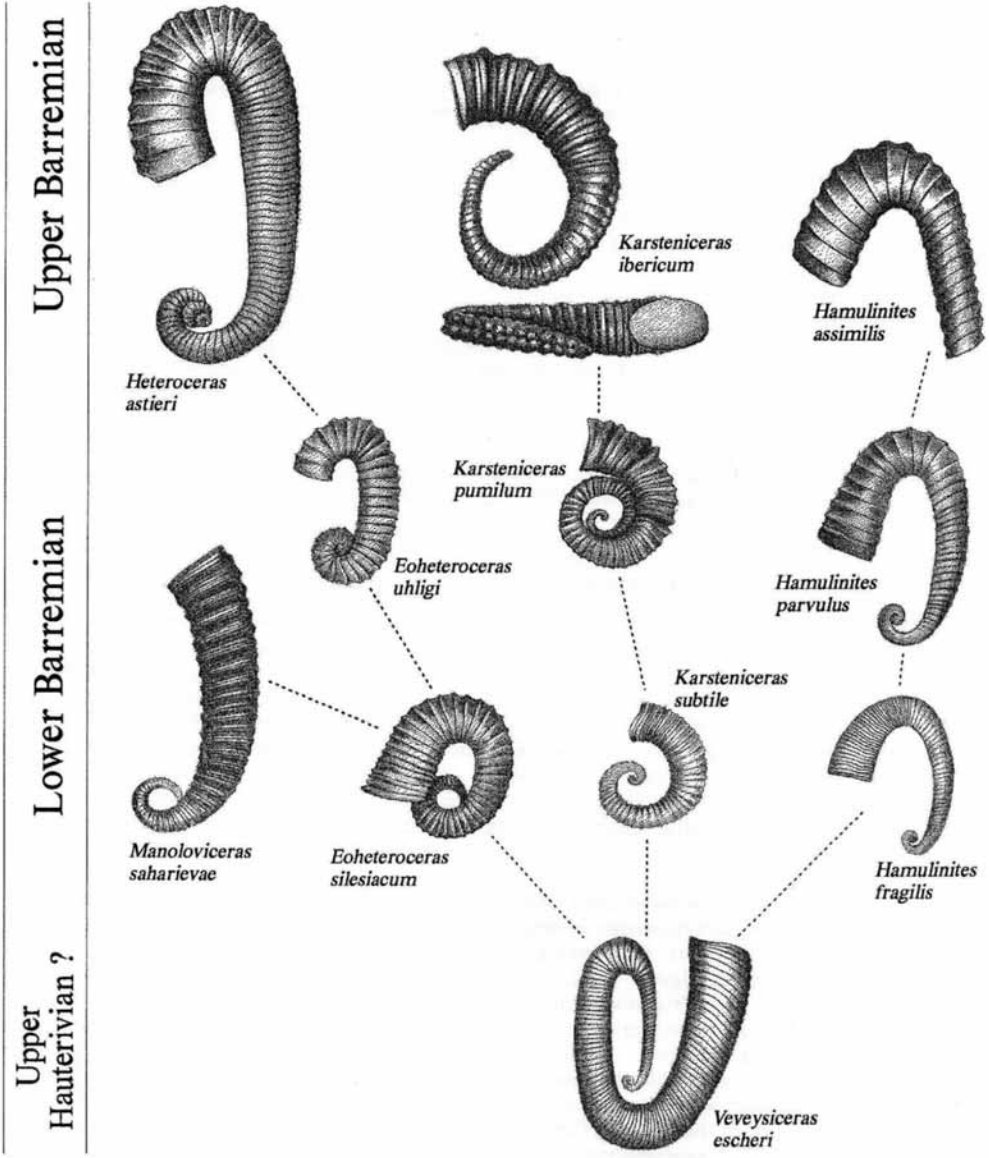
TEXT-FIG. 7. Evolution of Barremian Leptoceratoidinae.
