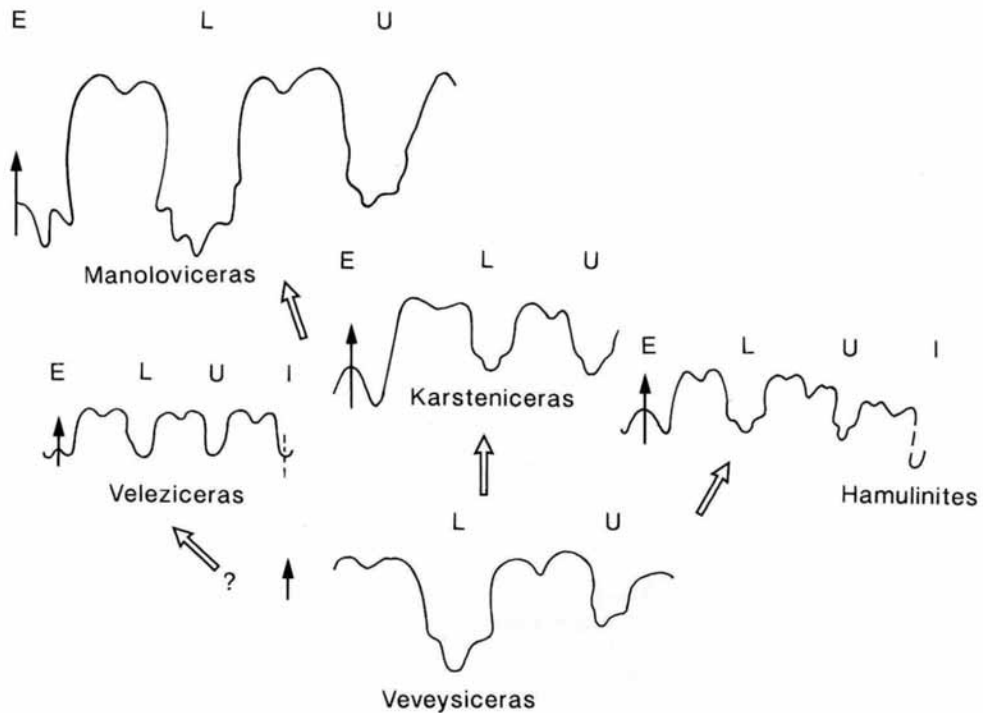
TEXT-FIG. 8. Evolutionary trends in adult suture-lines of the Leptoceratoidinae.
