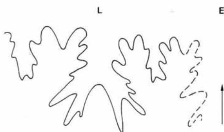
TEXT-FIG. 4. Fragmentary suture-line of Anahamulina distans Vašíček, at H = 6.5 mm; BSM AS III 452.
