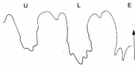
TEXT-FIG. 6. Fragmentary suture-line of Manoloviceras saharievae (Manolov) at H = 4.5 mm (after Vašíček 1972, fig. 19).
