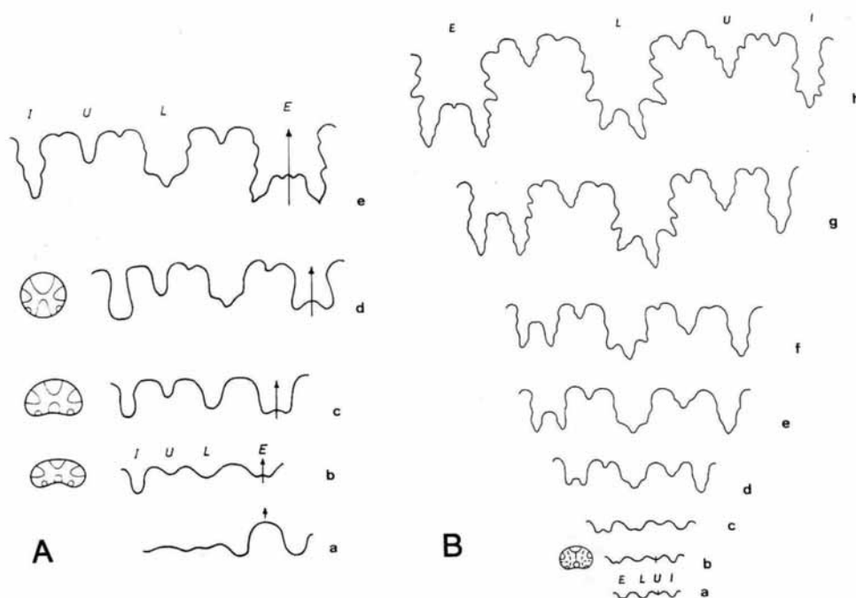
TEXT-FIG. 9. Comparison of suture ontogenies in leptoceratoids. A, Hamulinites parvulus (Uhlig) [= H. muniéri (Nicklès)], GPIT 1247/2; Lower Barremian; La Querola, Cocentaina, Spain; a, prosuture; b, primary suture and septal surface; c, at WH 0.5 mm; d, intermediate stage; e, at WH 2.5 mm (from Wiedmann 1963). B, Leptoceras studeri (Ooster), GPIT 1372/2; Berriasian; Rufisgraben-Jusital, Switzerland; a, primary suture; b, tenth suture and septal surface; c, 13th suture; d, 20th suture at WH 1.5 mm; e, intermediate stages; h, adult suture at WH 3.5 mm (from Wiedmann 1969).
