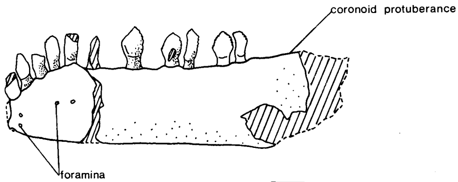
TEXT-FIG. 3. Azendohsaurus laaroussii Dutuit; t5 level; Azendoh, Morocco. MNHN-ALM 351, left dentary in external view, \times 1 . Scale bar = 10 mm.
