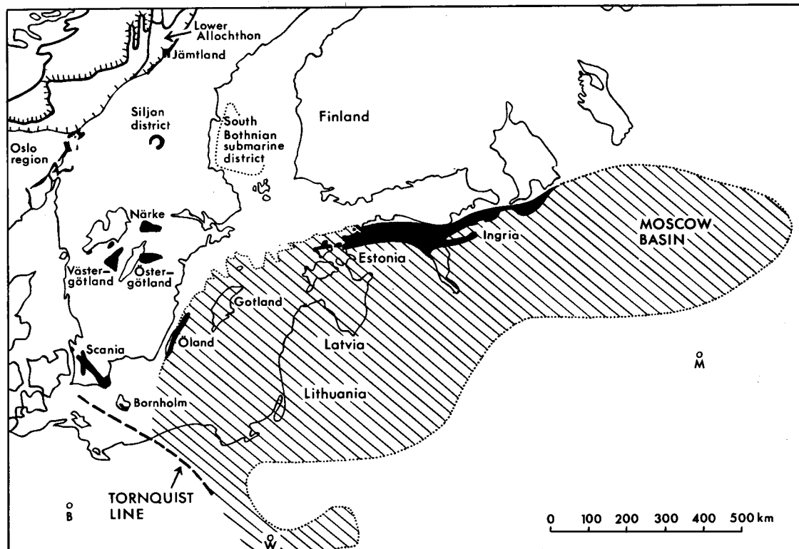
TEXT-FIG. 1. Districts of Ordovician outcrop in Baltoscandia (shaded black), and the extent of subsurface and submarine Ordovician on the Russian Platform (diagonal shading).
