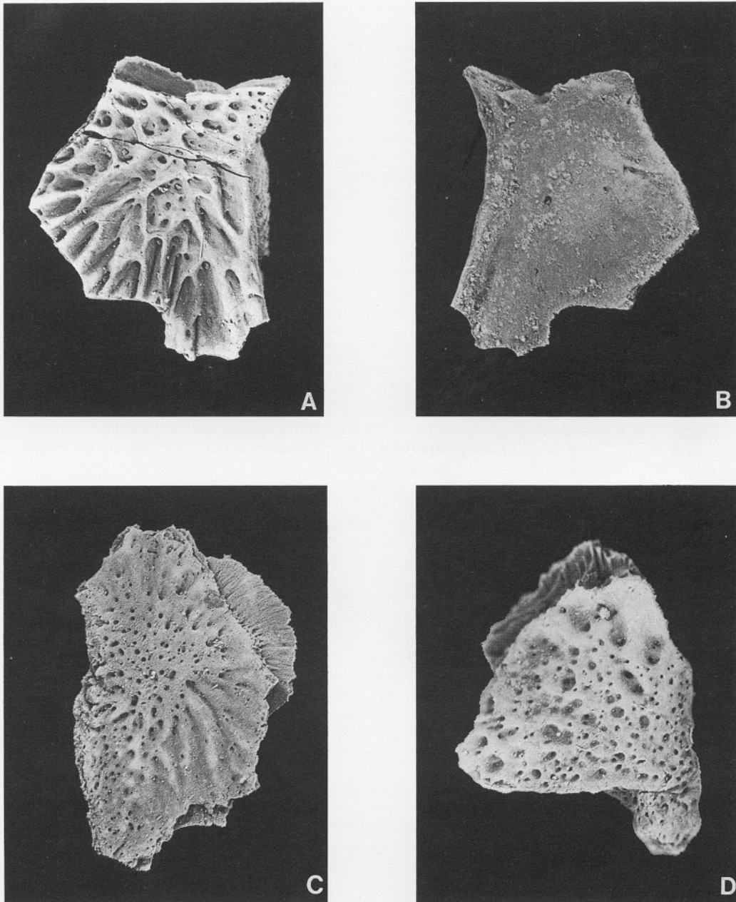
TEXT-FIG. 3. Undetermined tetrapod, cranial elements; Andreyevka; Famennian; A-B, PIN 2921/3002, right postorbital in dorsal and ventral views, \times 4 ; C, PIN 2921/3003, left intertemporal in dorsal view, \times 4 ; D, PIN 2921/447, right tabular in dorsal view, \times 10 .
