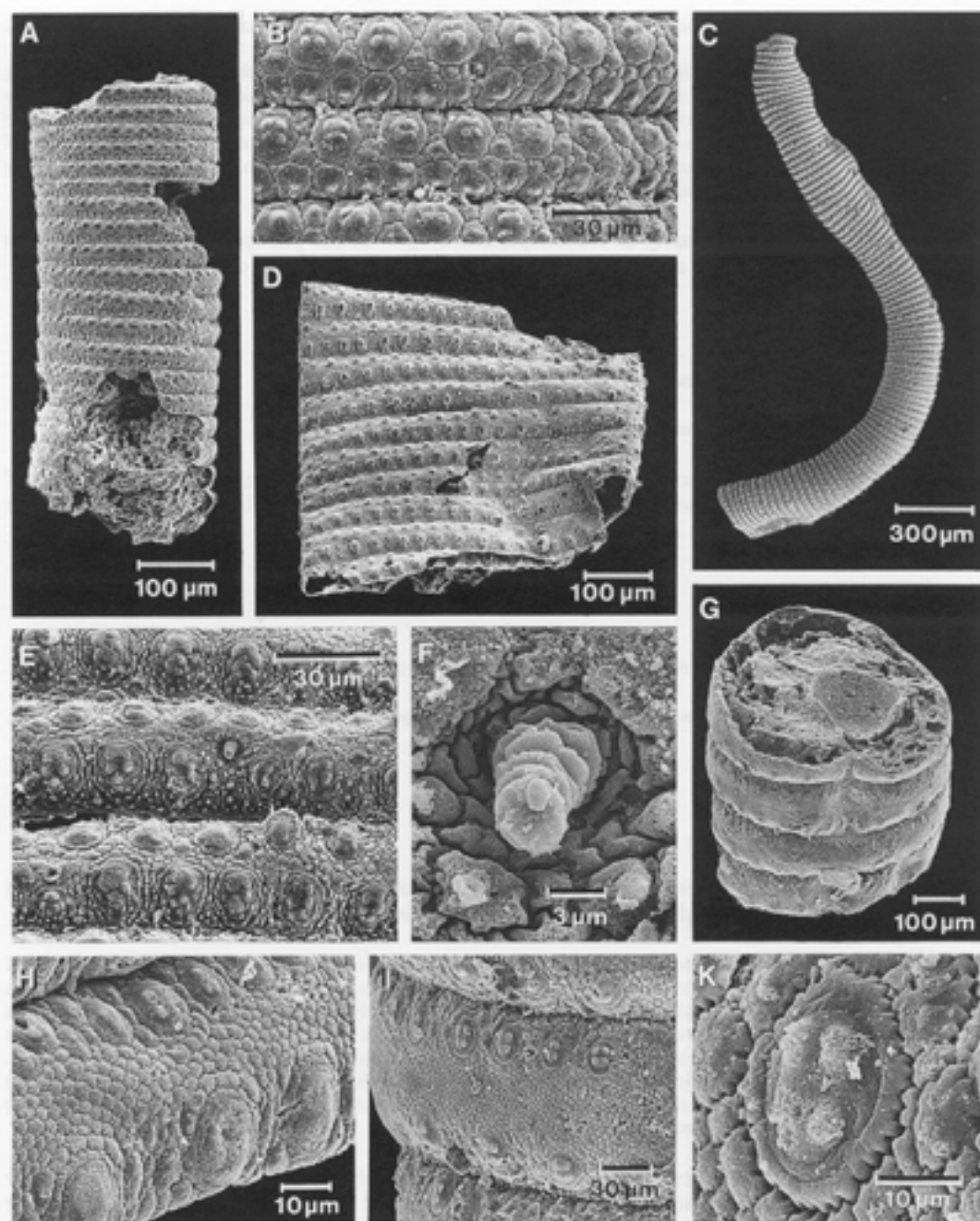
TEXT-FIG. 8. Murraysolex gen. nov. A-C, G-K, Murraysolex serratus sp. nov. A-B, CPC 23022 (sample 7390), holotype; Phosphate Hill, excavation no. 9, late Templetonian, Triplagnostus gibbus Zone. A, general view, \times 115 . B, detail of armour, \times 535 . C, CPC 23024 (sample 7337); 1 km north of Mt Murray (= D640), late Templetonian, Triplagnostus gibbus Zone; lateral view of curved specimen with broken aboral and oral ends,
