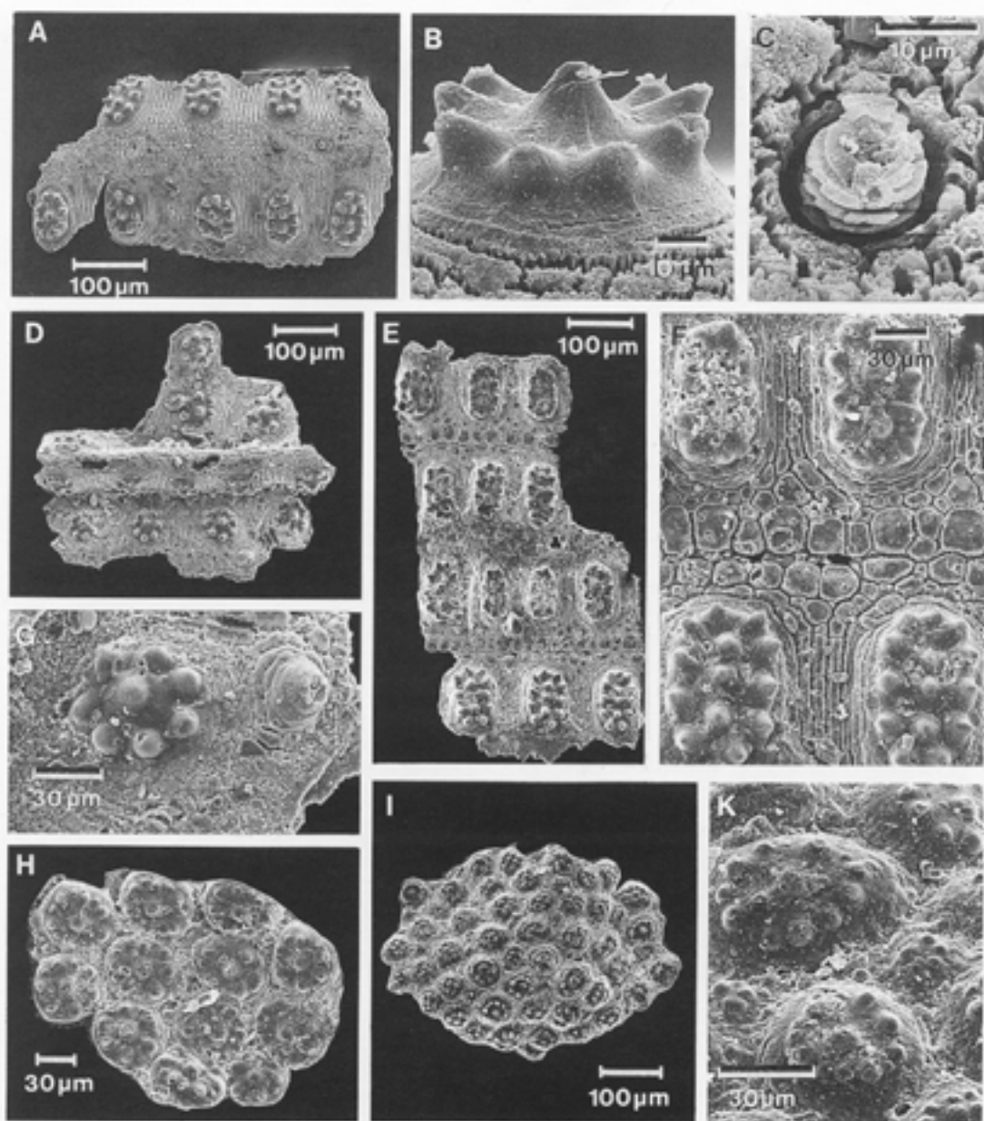
TEXT-FIG. 7. A-C, E-F, Milaculum elongatum sp. nov. A-C, CPC 23017 (sample 7336); 1 km north of Mt Murray, late Templetonian, Triplagnostus gibbus Zone. A, general view of fragment representing about the width of an annulus; note elongate platelets between plates, \times 110 . B, profile of single plate with fine radial ribs and jagged outer, basal margin, \times 800 . C, surface detail with broken tubule, \times 1550 . E-F, CPC 23018 (sample 7336), holotype; 1 km north of Mt Murray, late Templetonian, Triplagnostus gibbus Zone. E, piece of large specimen with broad, flat annuli, \times 100 . F, detail showing ornamentation of plates and mosaic pattern of platelets, \times 285 . D, G, aff. Hadimopanella oezguli form species I; CPC 23019 (sample 7324); Mt Murray, late Templetonian, Triplagnostus gibbus Zone. D, fragmentary, deformed specimen, \times 95 . G, detail of surface with plate and adjacent nipple-like protuberance, \times 365 . H-K, aff. Hadimopanella oezguli form species II. H, CPC 23020
