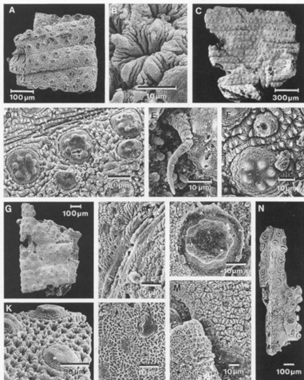
TEXT-FIG. 5. Corallioscolex gravius gen. et sp. nov. All specimens from 1 km north of Mt Murray (= D640), late Templetonian, Triplagnostus gibbus Zone, except where otherwise stated. A-B, D, CPC 23007 (sample 7336), holotype. A, general view of fragment, \times 110 . B, detail of coralliomorph outer surface with radially arranged platelets, \times 1900 . D, detail of armour with irregularly distributed plates; note folds at annulus border.
