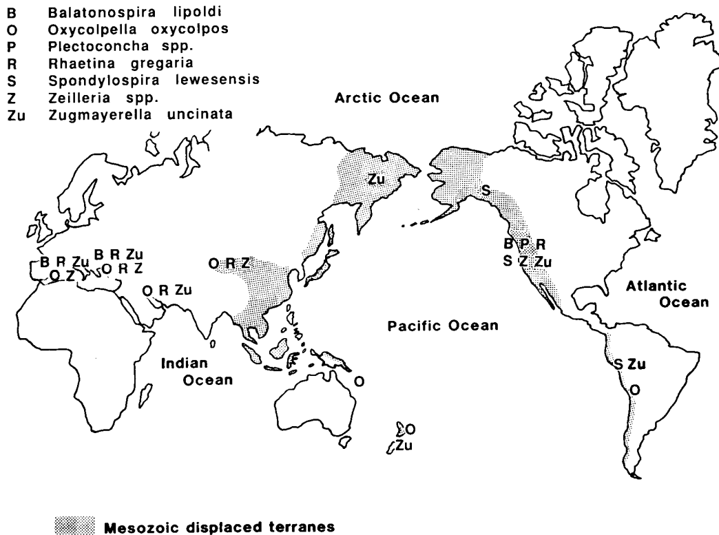
TEXT-FIG. 4. Map showing present-day geography and the distributions of brachiopod genera and species recorded from the Luning Formation, Nevada, and Oxycolpella (from Kristan-Tollmann 1987). Key to letters given in top left corner of figure. B = Balatonospira ? cf. B. lipoldi in Nevada. Sources of summaries of occurrence: Balatonospira lipoldi , Siblik 1988; Rhaetina gregaria , Pearson 1977; Spondylospira lewesensis , Hoover 1983, the genus has also been identified in the Koryak Range, north east former USSR; Zeilleria spp., Delancey 1974; Ching et al. 1979; Zugmayerella uncinata , Pearson 1977; and Oxycolpella oxycolpos , as interpreted by Kristan-Tollmann 1987. Map adapted from Stanley 1988.
