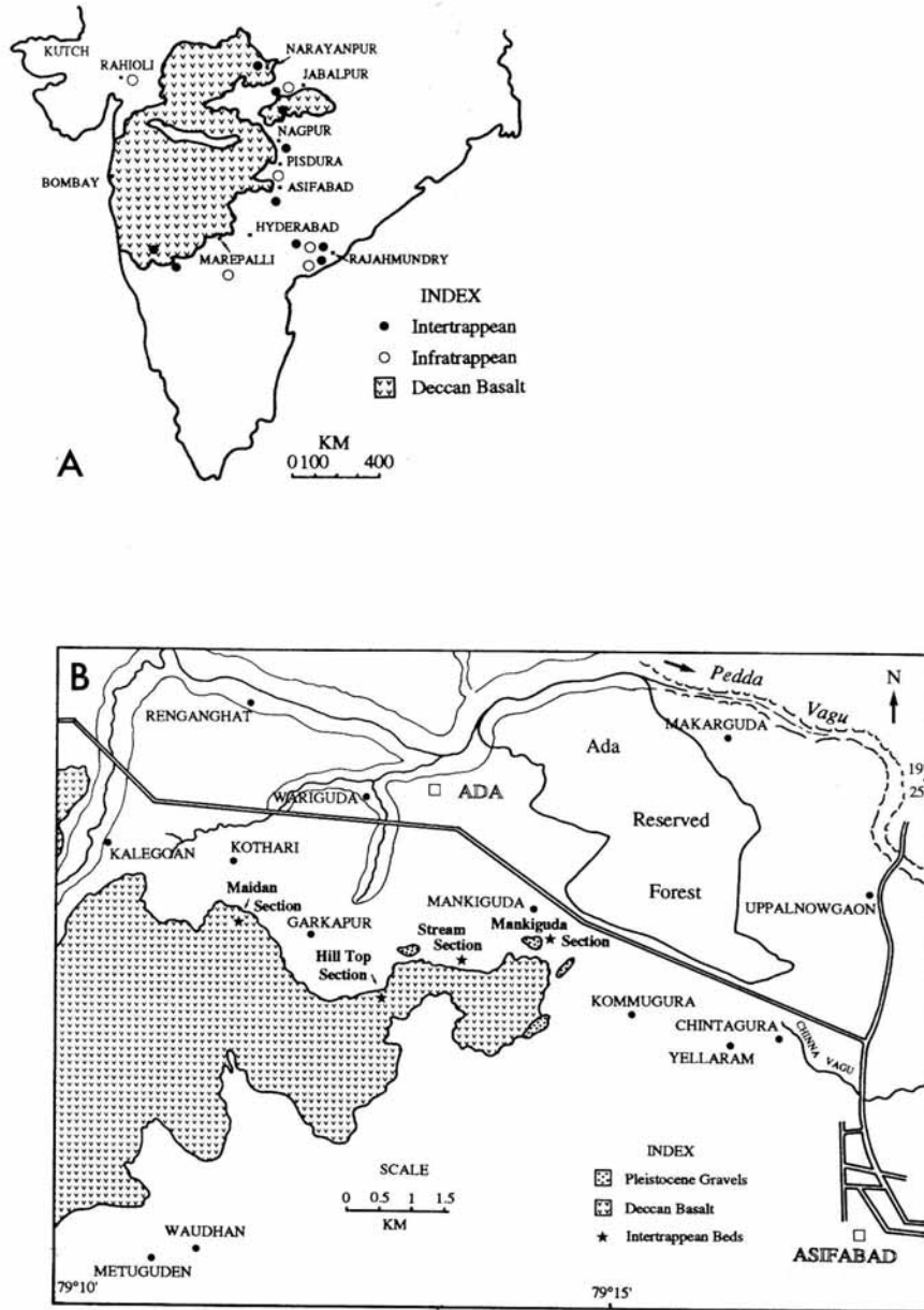
TEXT-FIG. 1. Location maps of the investigated localities. A, distribution of infra- and intertrappean beds in peninsular India. B, detailed locality map of Asifabad.
