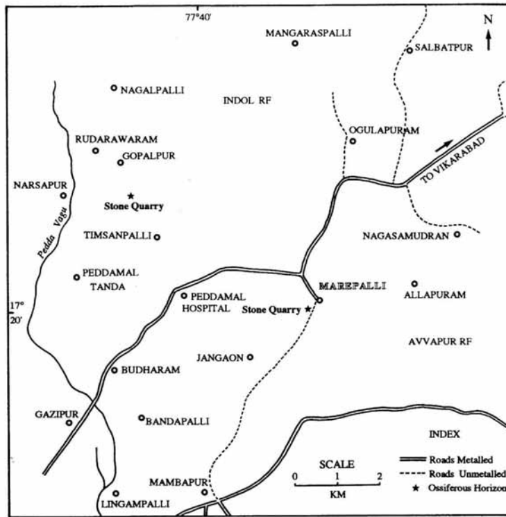
TEXT-FIG. 2. Detailed locality map of Marepalli.
