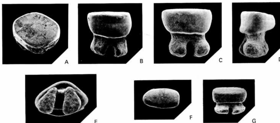
TEXT-FIG. 4. Rajiforme indet., Maastrichtian, intertrappean beds of Asifabad. A-B, VPL/JU 128; anterior tooth; occlusal and lingual views. C-E, VPL/JU 129; lateral tooth; lingual, profile and basal views. F-G, VPL/JU 130; very lateral tooth; occlusal and labial views. All figures \times 43 .
