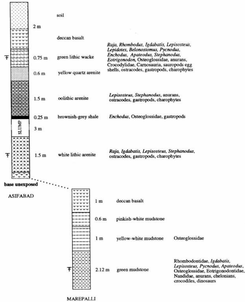
TEXT-FIG. 3. Stratigraphical columns of the ossiferous sections.
