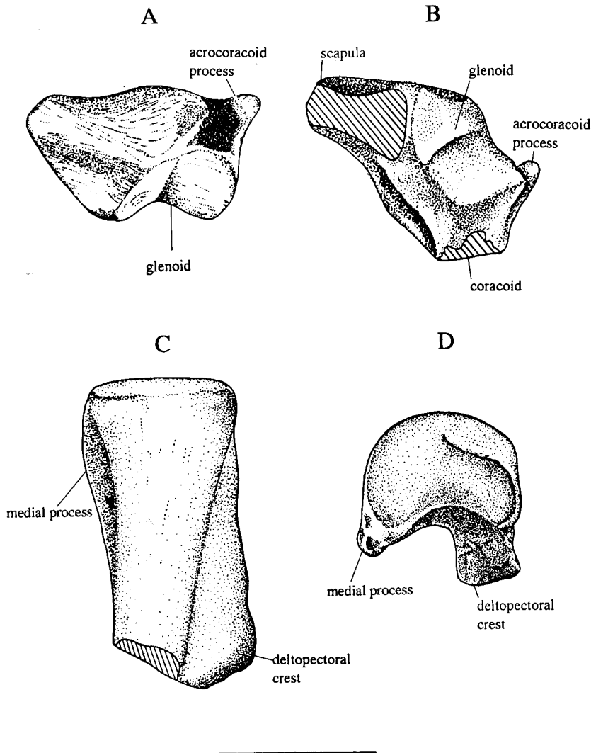
TEXT-FIG. 1. Santanadactylus brasiliensis . A–B, glenoid; positioned at the junction of scapula and coracoid, dorsal and lateral views. C–D, humerus only the proximal 40% of the shaft is preserved, dorsal and anterior views. Scale bar = 50 mm.
