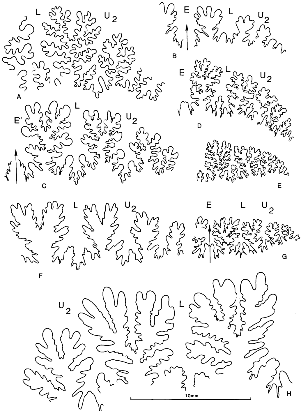
TEXT-FIG. 3. Sutures of A, Phylloceras ( Neophylloceras ) nera (Forbes, 1846), BMNH C22681. B, Saghalinites cala (Forbes, 1846), BMNH C51054. C, Phyllopachyceras forbesianum (d'Orbigny, 1850), BMNH C51080. D, Gaudryceras kayei (Forbes, 1846), BMNH C51050. E, Gaudryceras valudavurense (Kossmat, 1895), BMNH C51064. F, Desmophyllites diphyloides (Forbes, 1846), BMNH C22682. G, Pachydiscus ( Neodesmoceras ) soma (Forbes, 1846), BMNH C51039. H, Hauericeras rembda (Forbes, 1846), BMNH C51023.
