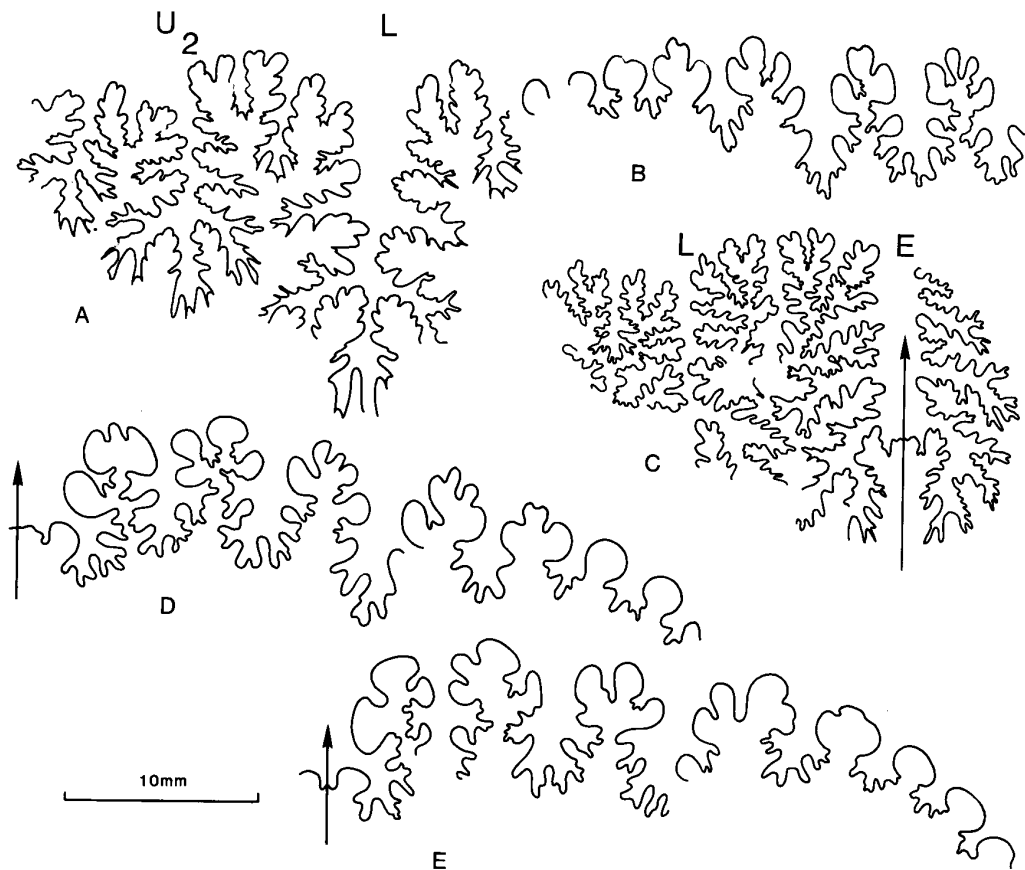
TEXT-FIG. 6. Sutures of A, Pachydiscus (Pachydiscus) neubergicus neubergicus (Hauer, 1858), the lectotype of Ammonites chrishna , Forbes, 1846, BMNH C51041. B, D, E, Sphenodiscus siva (Forbes, 1846). B, D, BMNH C51088, E, BMNH C51087, C, Menuites menu (Forbes, 1846), BMNH C47550.
