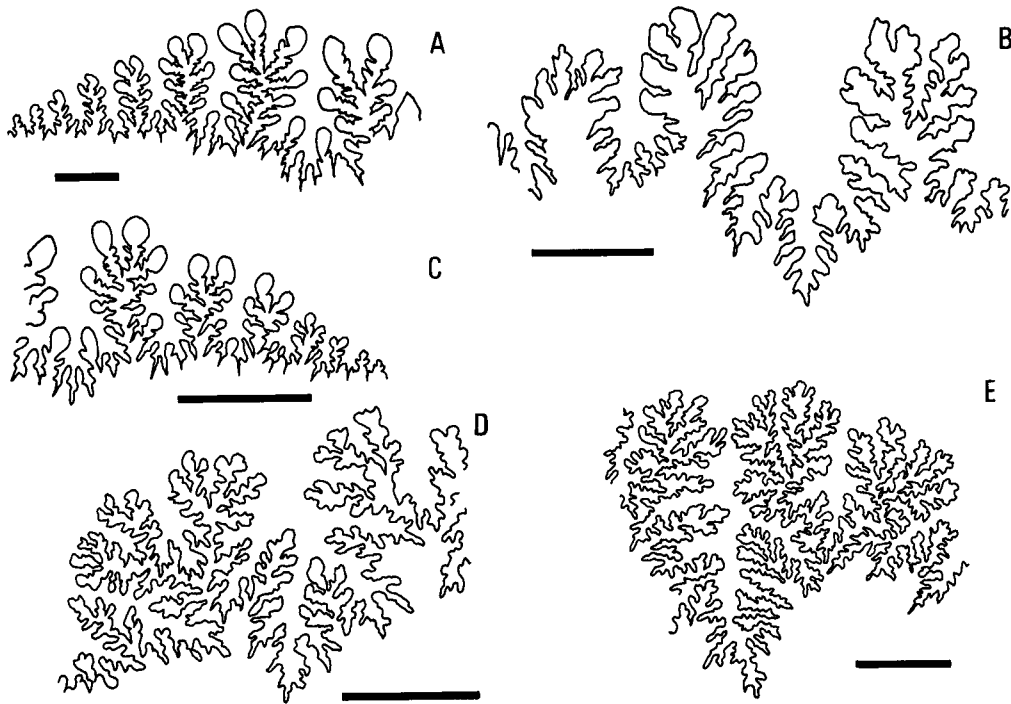
TEXT-FIG. 3. Suture lines of A, Calliphylloceras heterophylloides (Opper), J9477, Bed 1; B, Dorsetensia subsecta Buckman, J9494, Bed 6; C, Holcophylloceras zignodianum (d'Orbigny), J9486, Bed 1; D, Stephanoceras ( Stephanoceras ) scalare Weisert, J9472, Bed 10; E, Stephanoceras ( Stephanoceras ) triplex Weisert, J9497, Bed 10. Scale bars 10 mm.
