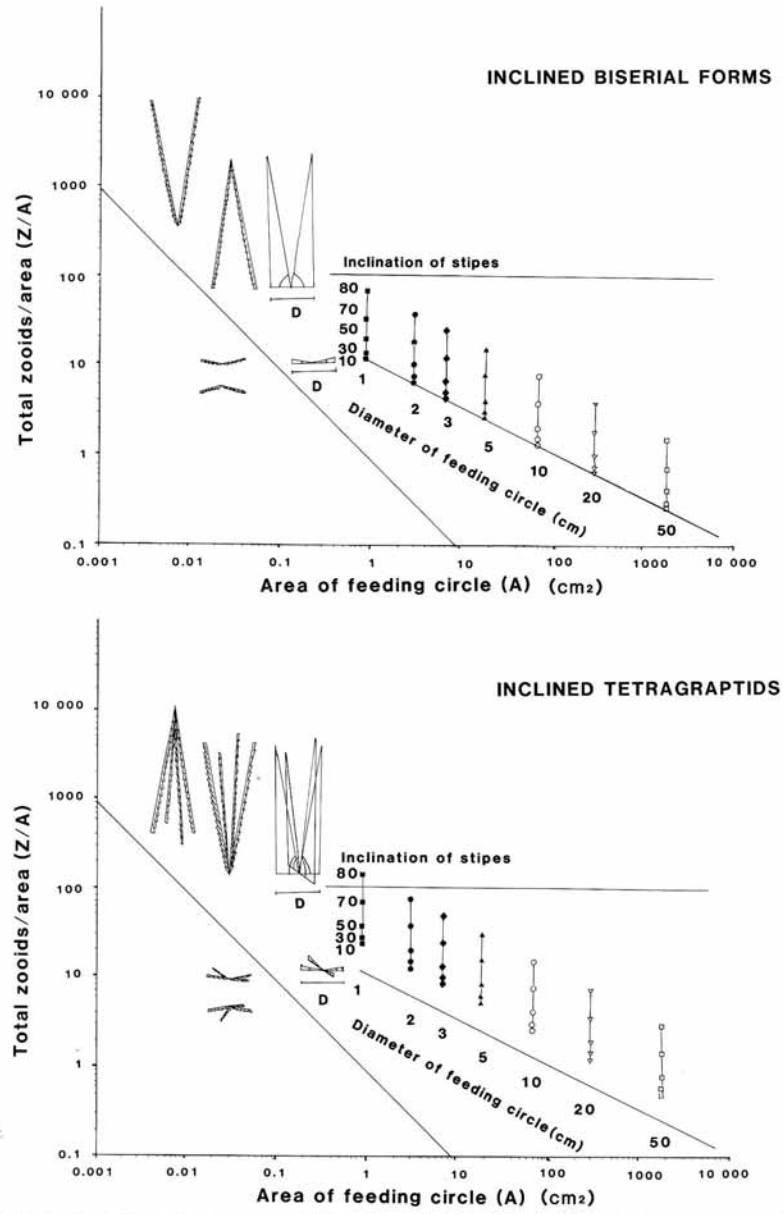
TEXT-FIG. 11. Inclined biserial and tetragraptid forms modelled mathematically with the region over which they plot on a feeding intensity - area graph shown.
