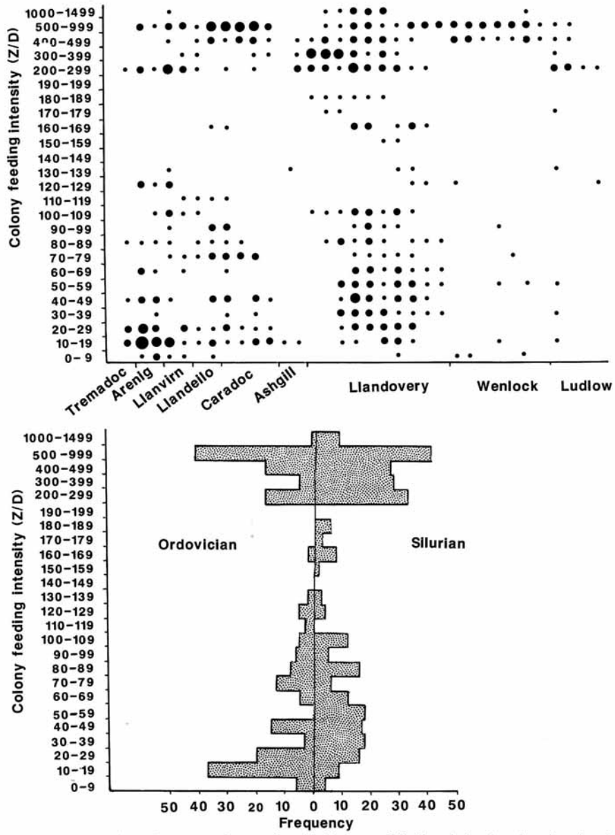
TEXT-FIG. 6. Feeding intensity, measured as total zooids/diameter of feeding circle, plotted against time (top) and summarized as a bar graph for the Ordovician and Silurian (bottom). Note that the change of scale at high feeding intensity values makes a false peak appear at the top of the bar graph. This is not a histogram.
