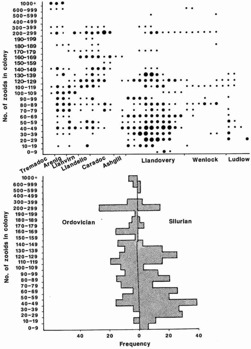
TEXT-FIG. 4. Total number of zooids in a colony plotted against time (top) and summarized as a bar graph for the Ordovician and Silurian (bottom).
