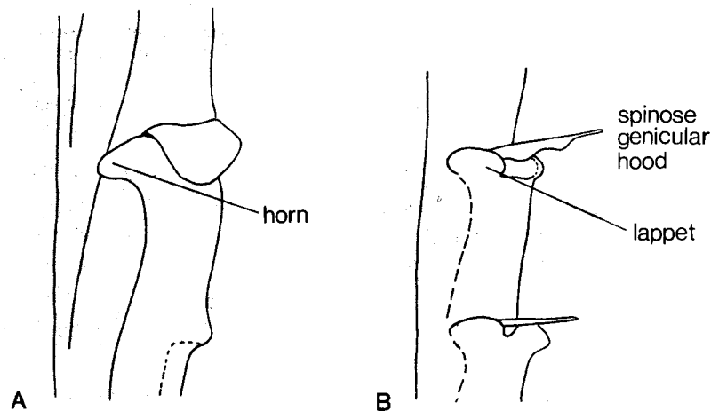
TEXT-FIG. 1. Prilylograptus leptotheca (Lapworth, 1876). A, internal mould of proximal theca (after Rickards and Rushton 1968, fig. 3). B, isolated proximal theca, UCWG926B. Both \times 25 .
