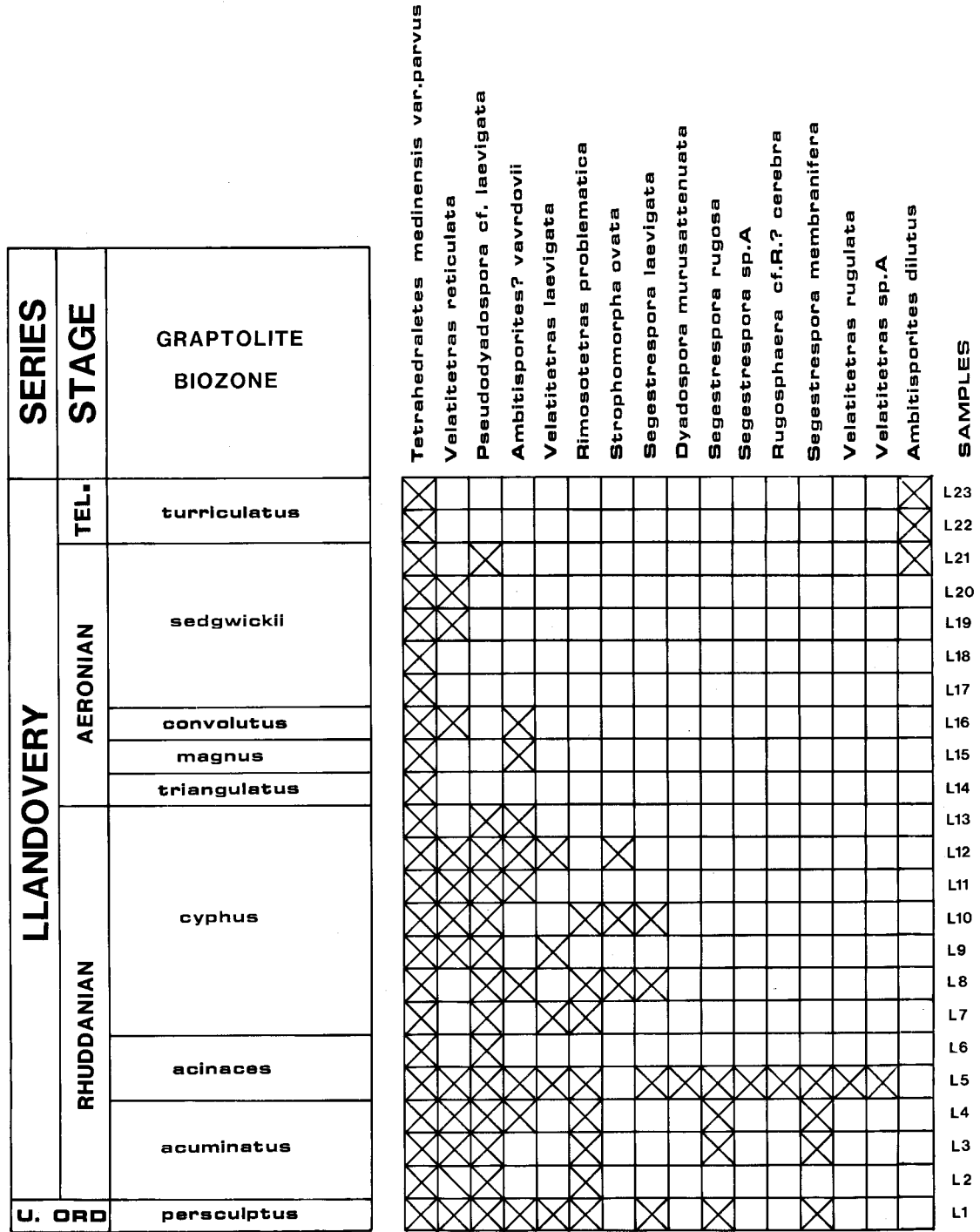
TEXT-FIG. 7. Biostratigraphic and lithostratigraphic ranges of sporomorphs from the type Llandovery area. Note that the majority of the Telychian was not sampled.
