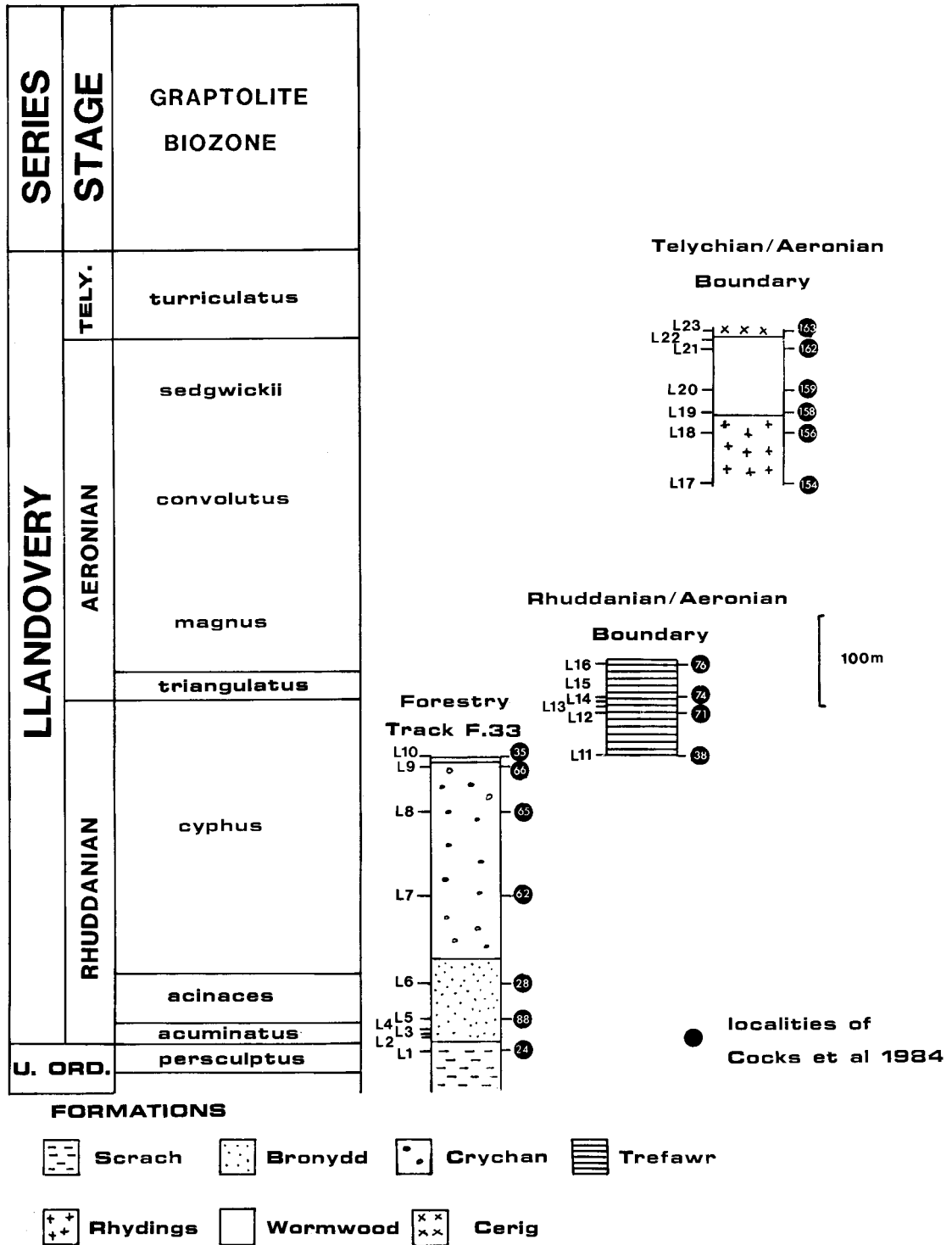
TEXT-FIG. 5. Biostratigraphic and lithostratigraphic position of samples from the type Llandovery area, in relation to localities of Cocks et al. (1984).
