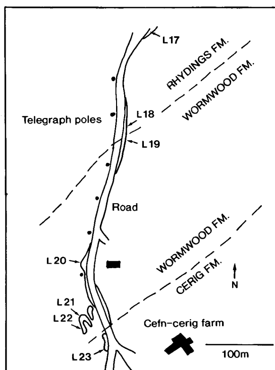
TEXT-FIG. 4. Locations of samples collected from the Aeronian/Telychian type boundary section in the type Llandoverly area: roadside near Cefn Cerig farm, near Llandoverly (Ordnance survey map reference SO 77543271 at sample L17 = locality 154 of Cocks et al. 1984).
