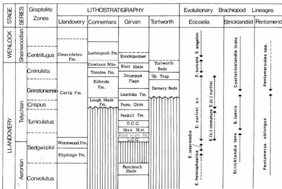
TEXT-FIG. 9. Lithostratigraphy of the Connemara, Girvan and Tortworth successions together with brachiopod lineages of relative value displayed relative to the current graptolite biostratigraphy and chronostratigraphy for relevant parts of the lower Silurian. Abbreviations: L.C.G., Lower Camregan Grits; Max. M.st., Maxwellston Mudstones; U.C.G., Upper Camregan Grits; Proto., Protovirgularia, Up., Upper.
