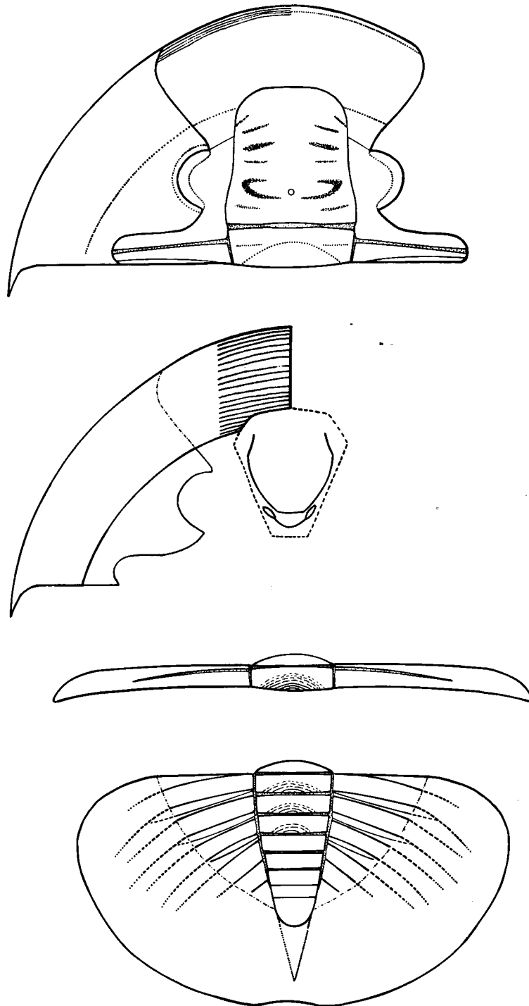
TEXT-FIG. 2. Restoration of Cermatops discoidalis (Salter), about \times 3 . Dorsal view of cranidium: the dorsal terrace-ridges are shown on the left side of the preglabellar field, the border furrow is indicated on the right. Ventral view of right free cheek and hypostome; terrace-ridges are shown on a representative area; hypostomal outline inferred (dashed), course of dorsal suture indicated (pecked). Dorsal view of thoracic segment. Dorsal view of pygidium.
