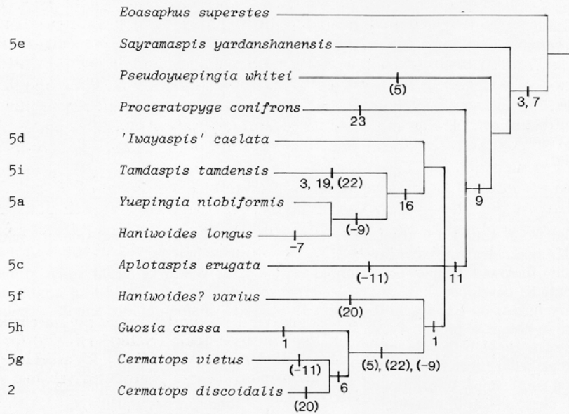
TEXT-FIG. 6. Relationships of selected taxa in the Iwayaspidinae, as indicated by the PAUP program (see text). Top, consensus tree with Proceratopyge conifrons for out-group comparison. Below, alternative tree with a hypothetical ancestor for out-group comparison. Eoasaphus is the most primitive actual taxon analysed. Numbers refer to characters in Table 1; negative numbers indicate character reversals and numbers in parentheses indicate parallelisms.
