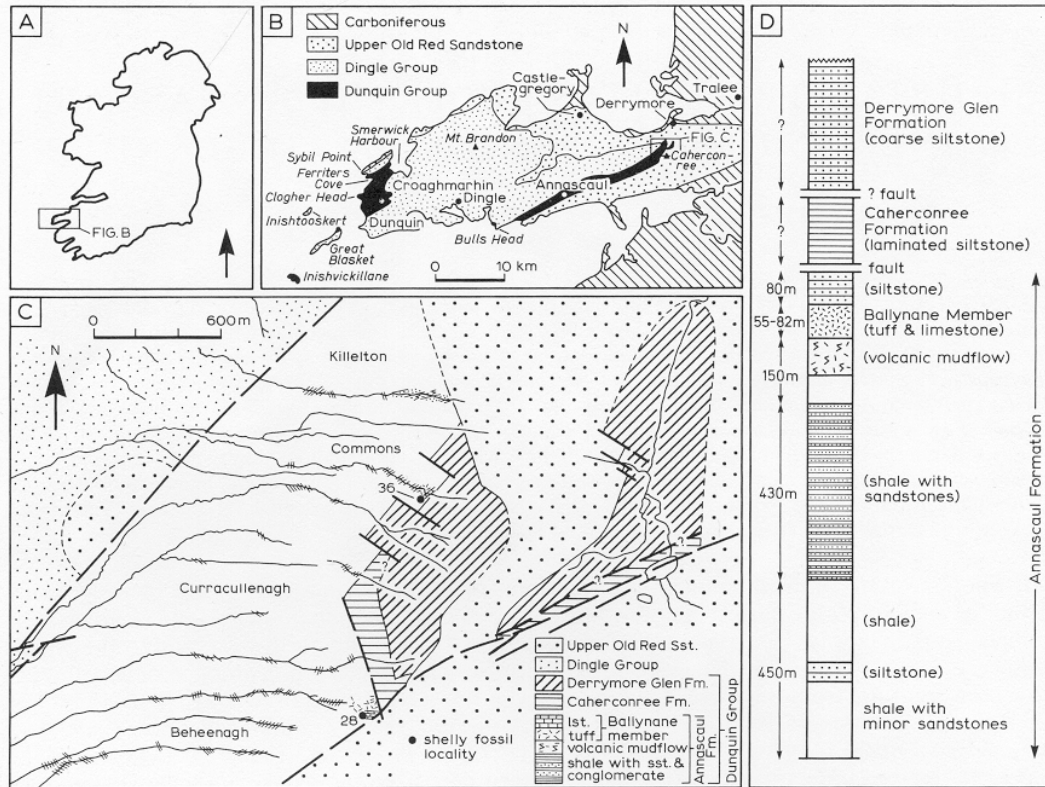
TEXT-FIG. 1. Locality map. A, Ireland with inset of the Dingle Peninsula. B, geological map of the Dingle Peninsula (after Holland 1981, fig. 48). C, geological map of the Carherconree-Derrymore Glen area, with the two fossil localities (28 and 36) which have yielded the trilobites described herein (simplified from Parkin 1976, fig. 4). D, stratigraphical section through the Dunquin Group, Bull's Head, Annascaul, and Derrymore Glen inliers (after Parkin 1976, fig. 5 and Holland 1981, fig. 49).
