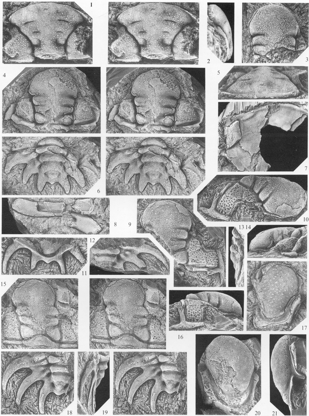
SIVETER, Silurian trilobites
