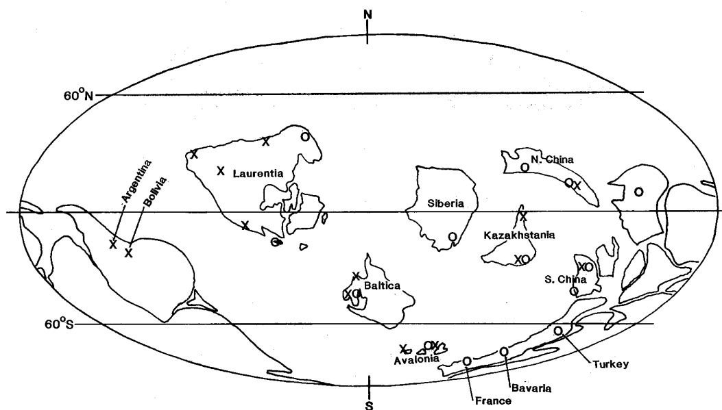
TEXT-FIG. 2. A global palaeogeographic reconstruction for the Tremadoc Series (modified from Scotese et al. 1979) showing the distribution of Parabolinella and Peltocare (crosses) and euolomids (rings).
