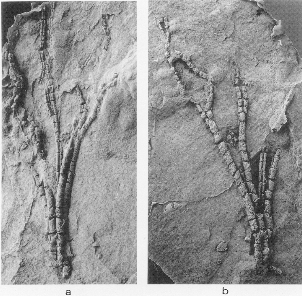
TEXT-FIG. 2. Photographs of latex moulds of Ramseyocrinus cambriensis from the Bolahaul Member, Ogof Hên Formation, Roman Road Section, Pensarn, Carmarthen, South Wales. a , crown NMW 86.93G.1 a showing arms, from left to right, B; A (branching and with food grooves); adoral view of C; E, crossing over D to form branches with food grooves at extreme right of figure; and D, branching with food grooves. Note circular cluster of plates between C and D arms at level of 1Br8 plates. \times 5 . b , crown of counterpart, NMW 86.93G.1 b . Food grooves are seen in the B and A rays and the arms in D and C rays are seen to branch. Note plate between arms D and C at level of 1Br4 plates, and cluster of plates between these arms at level of 1Br8 plates. \times 5 .
