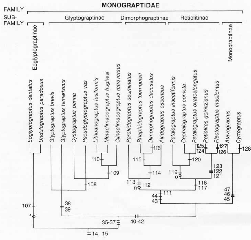
TEXT-FIG. 16. Cladogram and classification of the Monograptidae. Synapomorphies 1-61 as in text-fig. 13A; 107 , th^2 J-shaped and without upward growing flange in its prothecal ontogeny; 108 , thecal elongation to produce double sigmoidal curvature; 109 , undulatory median septum; 110 , thecal apertures hooded by overhanging genicular flanges; 111 , orthograptid thecae; 112 , strongly acicular proximal end with dorsal side of sicula free for nearly its entire length; 113 , metatheca of th^1 becomes upturned well above sicular aperture; 114 , metatheca of th^2 reduced; 115 , metatheca of th^2 absent but protheca retained; 116 , th^2 absent; 117 , thecae inclined at high angle to axis of rhabdosome and with everted aperture; 118 , th^1 and th^2 with concave ventral walls; 119 , rhabdosome aseptate; 120 , thecae elongate and with great overlap; 121 , ancora incorporated into thecal clathria; 122 , fusellar periderm reduced to clathria; 123 , metasicula suppressed; 124 , clathrial elements corresponding to edges of interthecal septa present; 125 , 'reticulum' that forms separate, lacinia-like mesh which encloses, but is free of, clathria along median region of rhabdosome; 126 , clathria lacks elements showing any clear correspondence with interthecal septa; 127 , reticulum entirely dependent on clathria; 128 , cladia present. Retained primitive character f as in text-fig. 13A; n , dicalyca th^2 ; o , fusellar periderm present.
