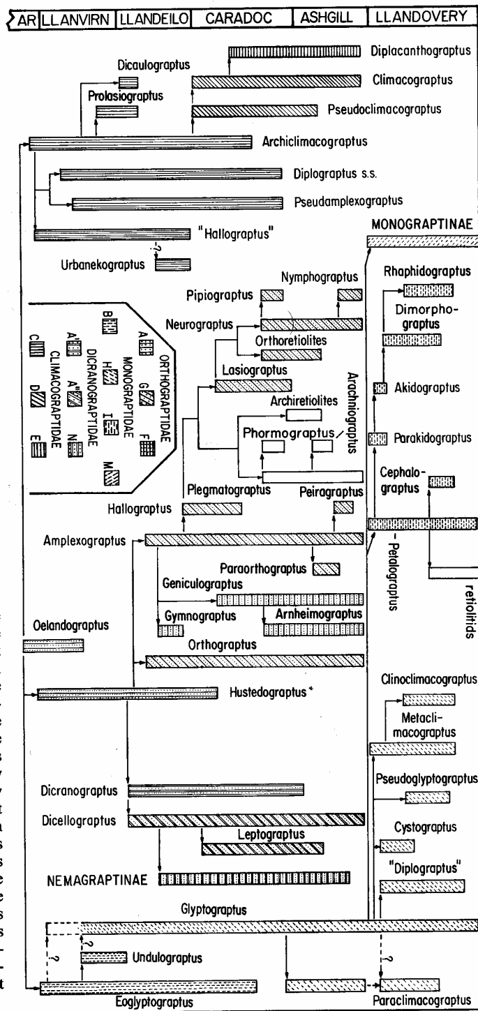
TEXT-FIG. 17. Evolutionary tree showing pattern of descent among the generic group taxa of the Diplograptacea in the interval of the upper Arerig to the base of the Wenlock Series. The nemagraptids and retiolitids are shown as family group taxa because of the remaining uncertainty about evolutionary relationships within them. The relationships among the generic group taxa of the Monograptinae are beyond the scope of the present study. Patterning within the range bars of each taxon indicates the astogenetic pattern exhibited by its constituent species and its family membership according to the inset key. The absence of patterning in range bars among the archiretiolitids (Orthograptidae) and retiolitids (Monograptidae) corresponds to the highly stylized clathrial architecture of these taxa that consequently does not fit within the astogenetic patterns defined herein. The plotted stratigraphic ranges of the taxa are approximate due to uncertainty about their species membership.
