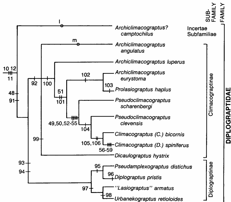
TEXT-FIG. 15. Cladogram and classification of the Diplograptidae. Synapomorphies 1–61 as in text-fig. 13A; 91, th1^1 and th1^2 with open curvature producing a broad, blunt proximal end; 92, metathecae of th1^1 and th1^2 with pronounced convex ventral walls and introverted apertures; 93, th1^1 and th1^2 with subhorizontal metathecae and generally with horizontal to everted apertures throughout; 94, 'amplexograptid' thecae with simple semicircular to introverted apertures and short, nearly vertical supragenicular walls; 95, straight median septum; 96, distal thecae orthograptid to glyptograptid; 97, genicular spines; 98, 'gymnograptid' thecae with well-defined clathria; 99, unique spinose dorsal margin of sicular aperture and with isolated, strongly introverted and spinose thecal apertures bearing fenestrate lateral processes; 100, flange of th2^1 formed on dorsal side of th1^2 ; 101, narrow, evenly rounded proximal end with tightly upturned th1^1 ; 102, open, semicircular apertures; 103, 'lasiograptid' thecae lacking genicular spines or lacinia but with clathria; 104, climacograptid thecae with relatively long, straight, and nearly vertical supragenicular wall; 105, straight median septum; 106, narrow, nearly parallel-sided rhabdosome. Retained primitive characters: l , archaic geometry of descending crossing canal of th2^1 along mid-line of colony in narrow proximal end; m , broad proximal end.
