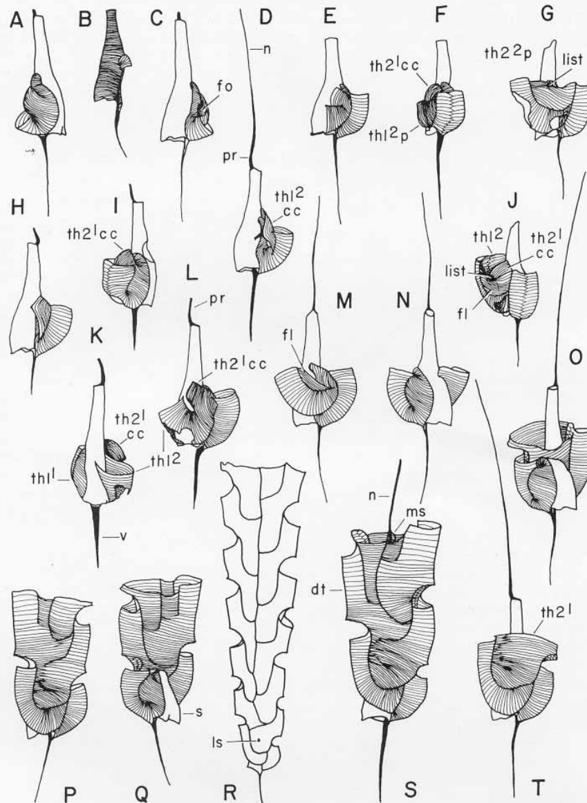
TEXT-FIG. 5. Camera lucida drawings illustrating Pattern D primordial astogeny in Climacograptus ( Climacograptus ) sp. cf. C. (C.) caudatus Lapworth; Viola Springs Formation (101 m above base of section H; Alberstadt 1973), Maysvillian Stage ( C. pygmaeus Zone), Arbuckle Mtns., Oklahoma. All illustrations are reverse views unless noted otherwise. See text-fig. 2 for explanation of abbreviations and specimen repositories.
