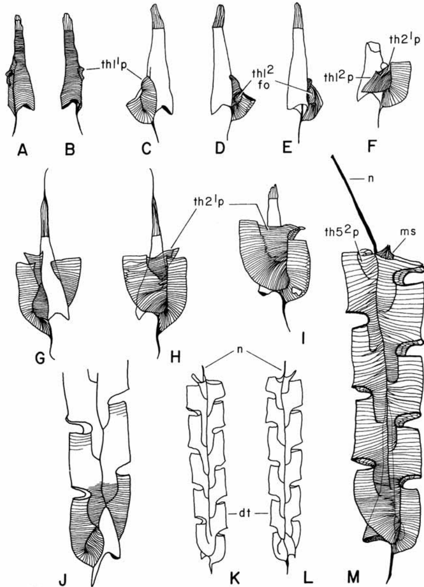
TEXT-FIG. 11. Camera lucida drawings illustrating Pattern H primordial astogeny in Glyptograptus kuckersi anus (Wiman); Kukruse Stage ( N. gracilis Zone), Estonia (Holm Collection). All illustrations are reverse view: unless noted otherwise. See text-fig. 2 for explanation of abbreviations and specimen repository.
