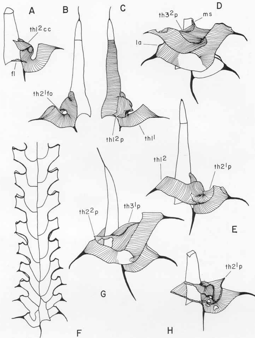
TEXT-FIG. 10. Camera lucida drawings illustrating Pattern G primordial astogeny in Amplexograptus bekkeri (Opik); Kukruse Stage ( N. gracilis Zone), Estonia (Holm Collection). All illustrations are reverse views unless noted otherwise. See text-fig. 2 for explanation of abbreviations and specimen repository.
