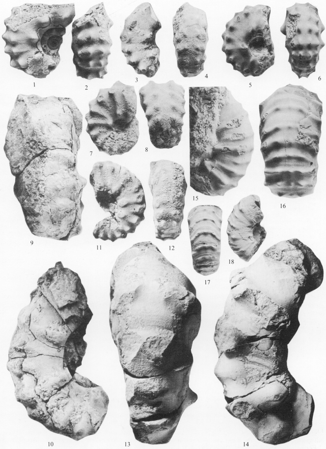
KENNEDY, WRIGHT and HANCOCK, Mammites , Kamerunoceras
