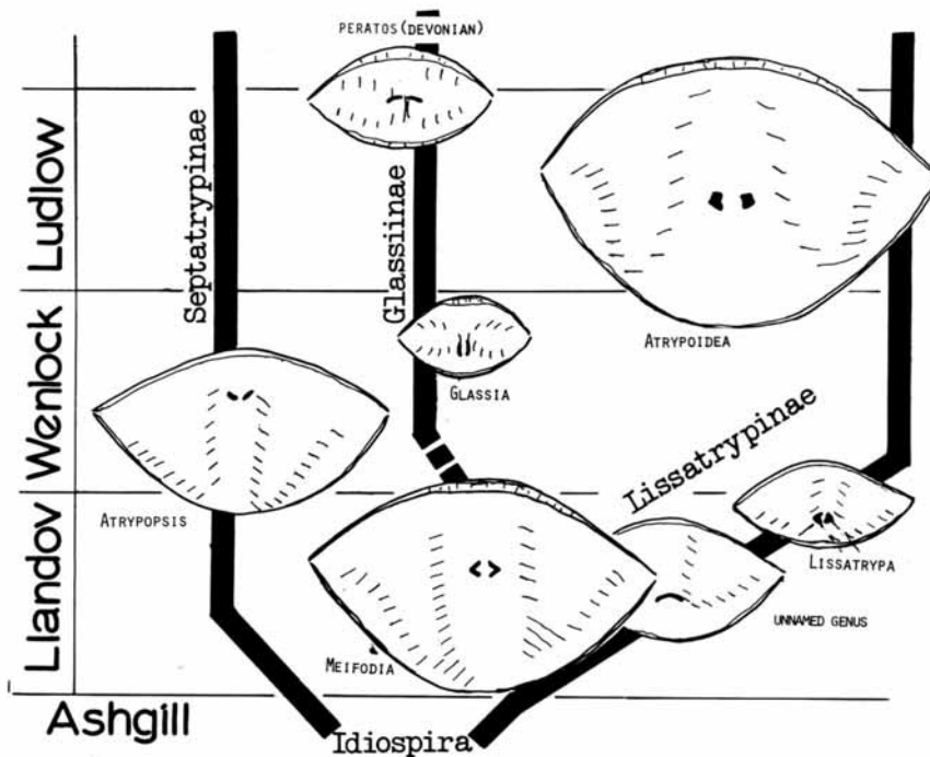
TEXT-FIG. 3. Nature of the jugum and spiralia in the Silurian Lissatrypidae subfamilies. Representative serial sections shown were taken at maximum spiralia size. The ends of the jugal processes, i.e. usually the jugal plates, are superimposed on these serial sections although these normally do not extend to mid-shell. Note that all Silurian smooth atrypoids have separated jugal processes but for one un-named new genus from Anticosti. All specimens to scale of \times 2 .
