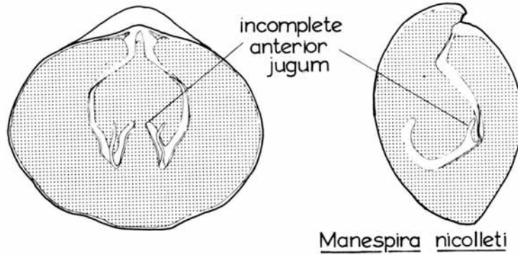
TEXT-FIG. 6. Brachidia of Manespira nicolleti (Winchell and Schuchert, 1892), based on text-fig. 7. Note the incomplete jugum and delicate half-whorl of the spirialium. Scale \times 10 .
