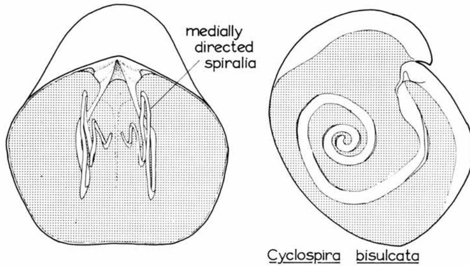
TEXT-FIG. 11. Brachidia of Cyclospira bisulcata (Emmons, 1842), based on text-fig. 13. Note the medial direction of spiralia and absence of a jugum. Scale \times 10 .
