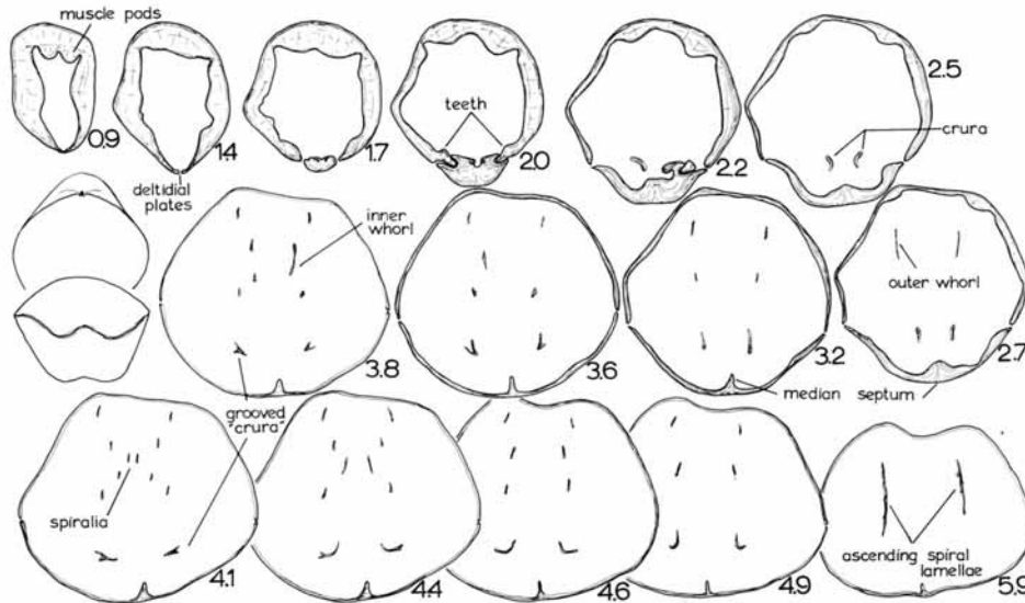
TEXT-FIG. 13. Serial sections of Cyclospira bisulcata (Emmons, 1842) from the designated type locality, 600 m east-north-east of Rodman, along Gulf Stream, NY; Hillier Mbr, Cobourg Fm., late Caradoc, lower CF11. GS79442. Scale \times 5 .
