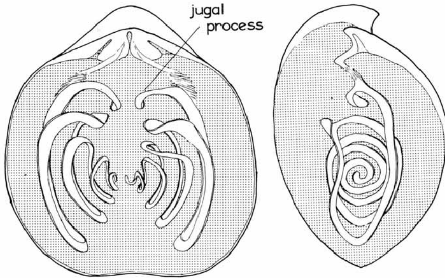
TEXT-FIG. 14. Brachidia of Glassia elongata Davidson, 1881, based on text-fig. 15. Note that crura are fibrous, jugal processes separated and spiralia curved in the centre. Scale \times 8 .
