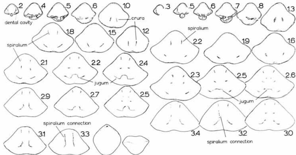
TEXT-FIG. 5. Serial sections of two specimens of Protozyga exigua (Hall, 1847). Napanee Limestone, near Napanee, Ontario, NTS 31C/7W 44600:02930; Caradoc, Harnagian-Soudleyan. Note that spirallium connection occurs near the anterior commissure. Scale \times 4 .
