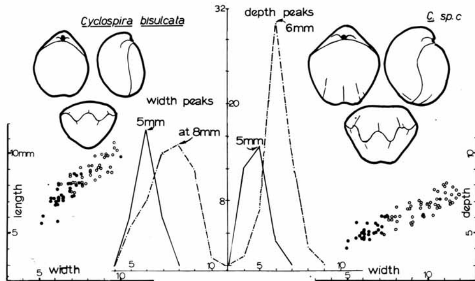
TEXT-FIG. 12. Scatter diagrams and frequency curves comparing Cyclospira bisulcata (shown on left, solid dots, solid lines) from Gulf Stream, NY with an undescribed sp. C (circles, dashed line) from the upper Cobourg Fm., Craigeath, Ontario which is believed to represent a stratigraphically younger form (high CF11).
