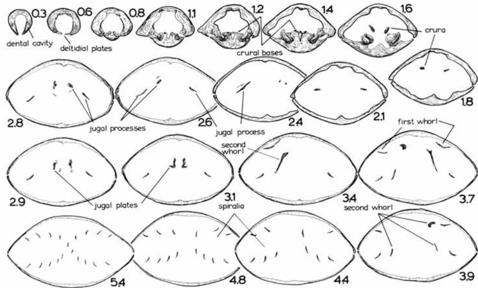
TEXT-FIG. 15. Serial sections of Glassia elongata Davidson, 1881 from the lower Mulde Beds, Djupvik 2, 61 Visby SO 41660:55730, Gotland, Sweden; middle Wenlockian. A dental cavity is present posteriorly, but dental plates are absent; spiralia are barrel-shaped instead of conical. GS79444. Scale \times 4 .
