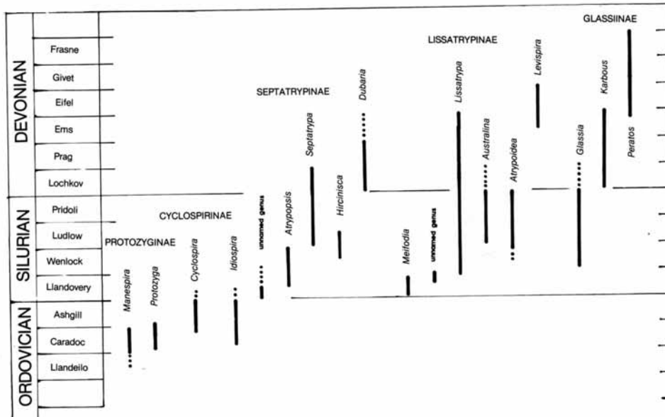
TEXT-FIG. 18. Stratigraphic distribution of known genera and subfamilies of smooth atrypoid brachiopods from Ordovician through Devonian time. The genera Nanospira , Lissatrypaidea , and Tyrothyris are taken as synonyms of Australina . Buceqia Havlicek and Quangyuania Sheng are interpreted as probable synonyms of Lissatrypa . Cryptatrypa is a synonym of Glassia . The smooth brachiopod Manosia Zeng is a genus whose affinity is uncertain. The genus Holynatrypa is also of very uncertain status. Synonymous and dubious genera are not included in the range chart.
