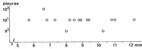
TEXT-FIG. 8. Number of pygidial pleurae plotted against pygidial length (articulating half-ring excluded) in Balizoma obtusus Form B. There is no correlation between size and number of pleurae. All specimens from Hulte 3 (Ar52337, Ar52423-52436).
