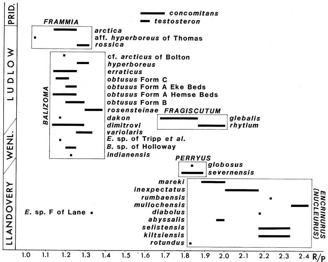
TEXT-FIG. 3. R/P ratios for certain encrinurids. The species are arranged approximately chronologically, but there are probably several errors due to poor data. Each supraspecific taxon has a limited range of the R/P ratio and a restricted vertical distribution. Authorships of the species are given in the discussions of Balizoma and Encrinurus ( Nucleurus ).
