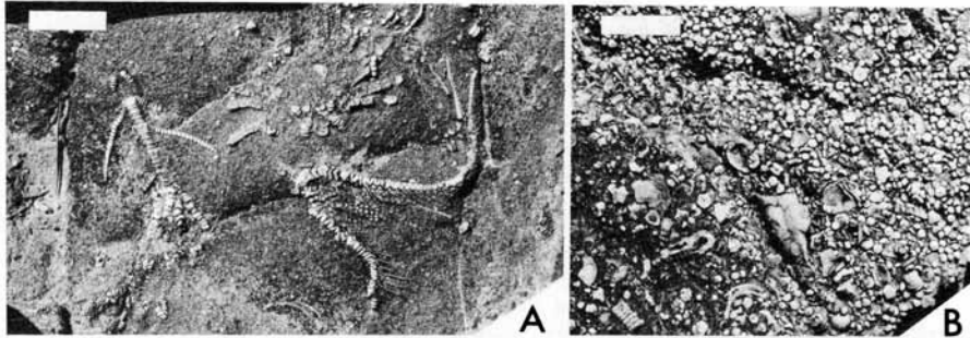
TEXT-FIG. 3. Mode of occurrence of Isocrinus (Chladocrinus) hanaï sp. nov. at Loc. Hn 0920, northern coast of Haïpe. A, well-preserved specimens in fine-grained sandstone. B, slightly below the horizon of A, consisting mostly of cirrals. Both figures are views of bedding plane surfaces. Scale bars 2 cm.
