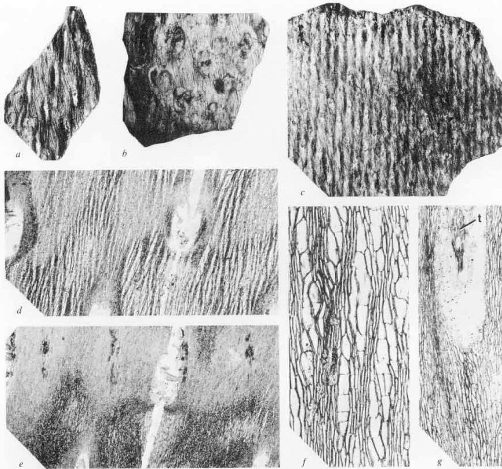
TEXT-FIG. 2a-g. Chaloneria cormosa cortex in surface views and in tangential sections; t, leaf trace. a, cortex of specimen with well-developed periderm, split at level of 'd' in Plate 64, fig. 2, C.B. 2126, \times 1 . b, cortex of same specimen as a, but with leaf bases split slightly further toward periphery, at level comparable to specimen in Plate 64, fig. 5, C.B. 2126, \times 1 . c, surface of cortex at level similar to that in Plate 64, fig. 1, but from specimen with only limited periderm, comparable to outer surface of cortex at bottom of Plate 64, fig. 4, C.B. 2126, \times 1 . d, tangential section through cortex of specimen with significant periderm, comparable to surface in b, C.B. 2127A(1) Side no. 6, \times 2.5 . e, tangential section through periderm of specimen in d showing anatomical derivation of Knorria configuration, C.B. 2127A(1) side no. 9, \times 2.5 . f, enlargement of anatomical detail in d, C.B. 2127 no. 7, \times 17 . g, enlargement showing anatomical detail of tissue that compresses to produce Knorria configuration, C.B. 1398D(1) side no. 310, \times 17 .
