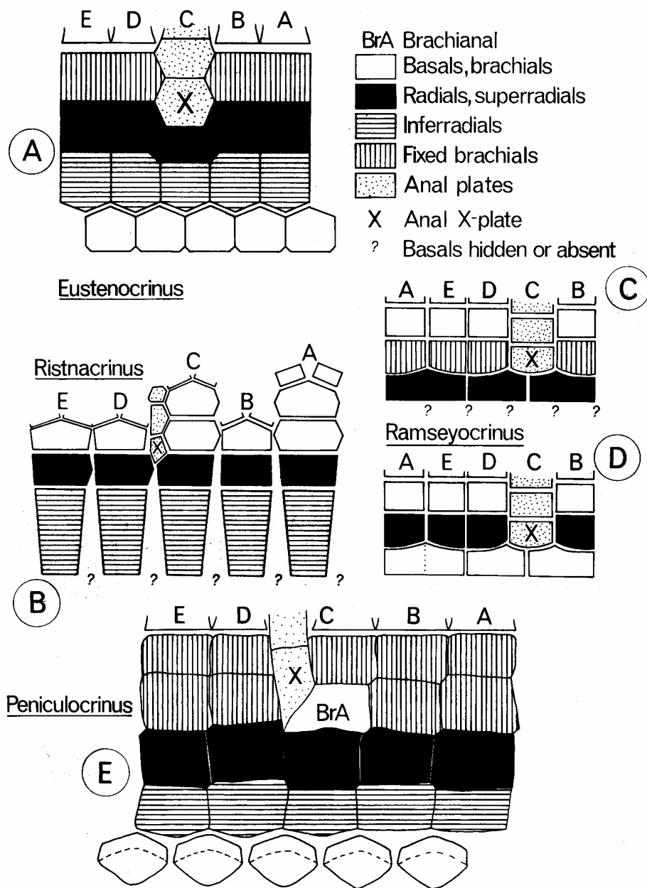
TEXT-FIG. 1. Cup plating diagrams for: A, Eustenocrinus (after Ulrich 1925; Moore 1962); B, Ristnacrinus (after Öpik 1934); C, D, Ramseyocrinus . Two interpretations of the cup are shown, both based on NMW 29.308.G296 and G318 (counterparts). In C the basals are hidden or absent, radials and a circlet of fixed brachials are present, and the anal X is supported by two radials (this paper). In D basals and radials are present, two basals supporting the anal X (based on the description of Bates 1968). E, Peniculocrinus (after Moore 1962).
