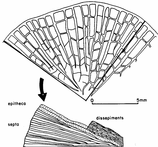
TEXT-FIG. 7. Part of a thecosmilian cross-section to illustrate method used for estimating proportion of skeleton per unit area of corallite.
