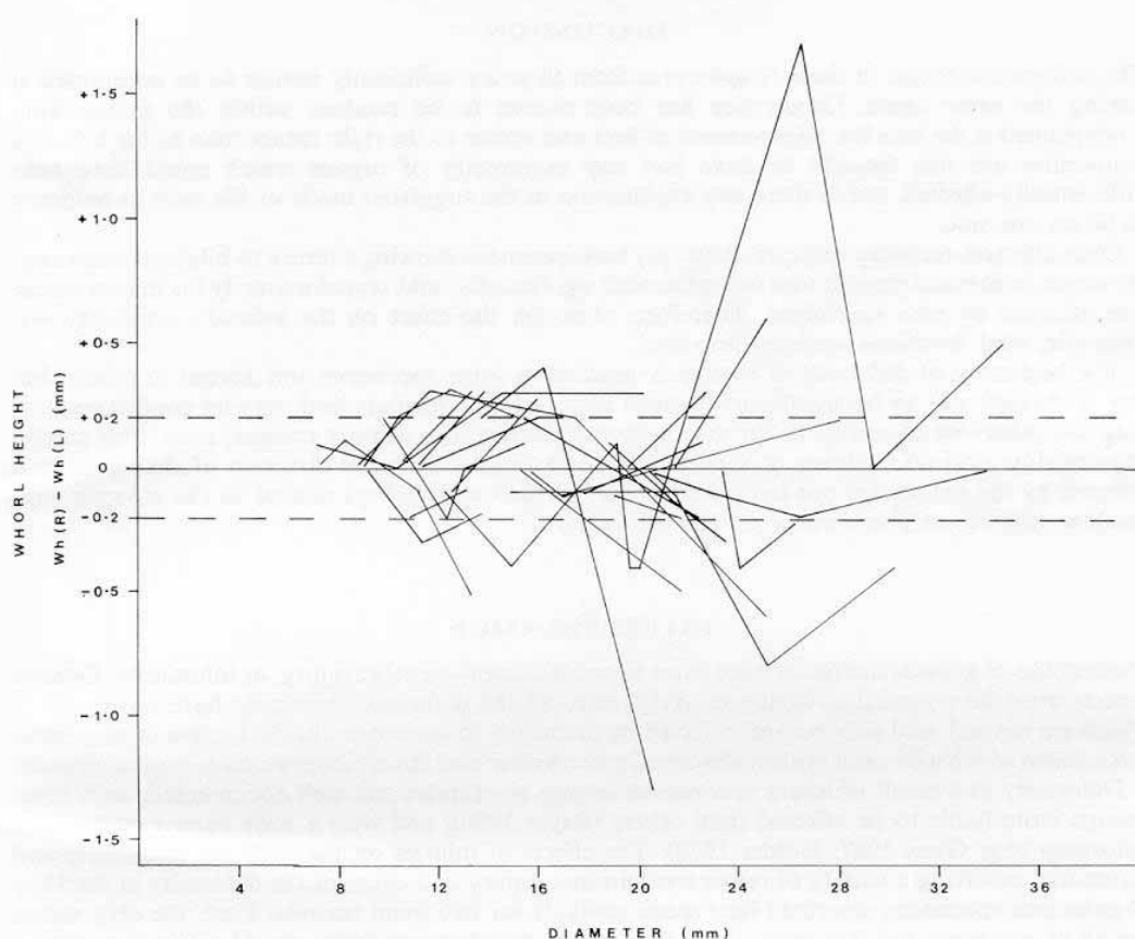
TEXT-FIG. 4. Deformity of Graphoceras from the concovum Zone, Berreraig, Skye; loss of bilateral symmetry of whorl cross-section measured as the difference in whorl height on either side, by subtracting Wh. on the left side from Wh. on the right side at the same position (Right/Left convention explained in text). A difference of more than 0.2 mm results in visible asymmetry of the whorl cross-section.
