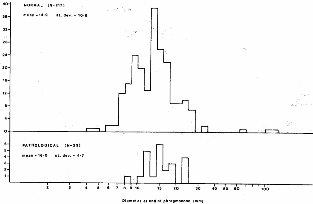
TEXT-FIG. 1. Size-frequency distribution of normal and pathological ammonites, Graphoceras aff. concauum (Buckman), concauum Zone, Bearreraig, Skye.
