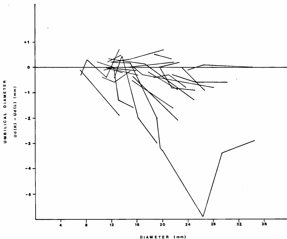
TEXT-FIG. 3. Deformity of Graphoceras from the concavum Zone, Berreraig, Skye; loss of bilateral symmetry measured as the effect on umbilical diameter by subtracting Ud. on the left side from Ud. on the right side at the same position (Right/Left convention explained in text).
