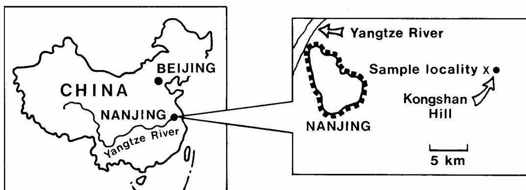
TEXT-FIG. 1. Location of Kongshan Hill, near Nanjing.
