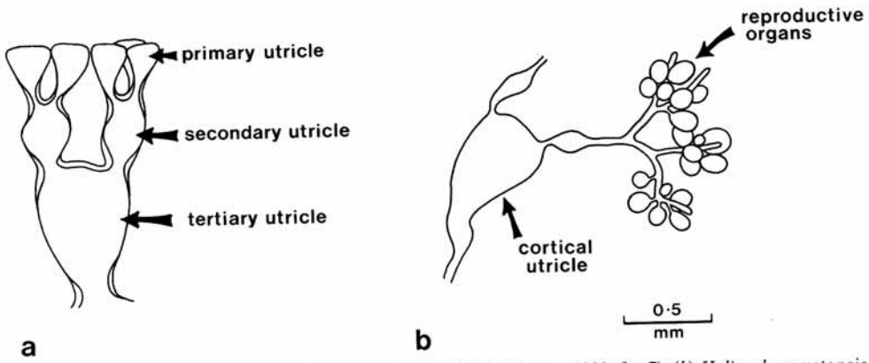
TEXT-FIG. 10. (a) Halimeda , utricles in the cortex (from Hillis-Colinvaux 1980, fig. 7). (b) Halimeda gametangia forming clusters on filamentous extensions of the cortical utricle (from Egerod 1952, fig. 19c).
