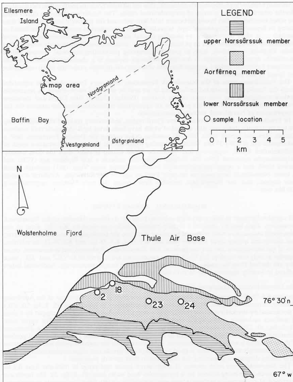
TEXT-FIG. 1. Locality map of the Narssârssuk Formation.
