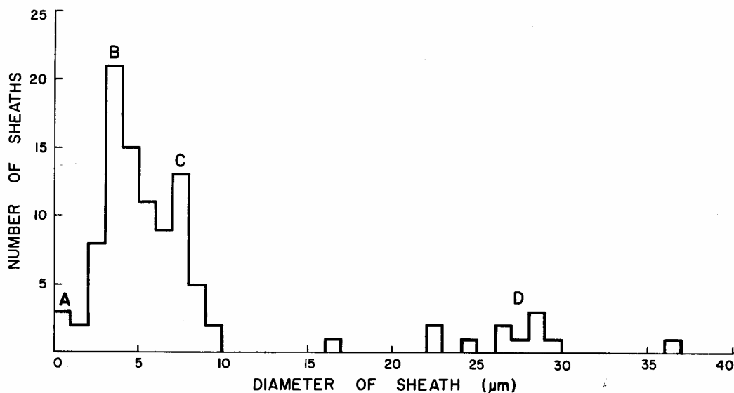
TEXT-FIG. 4. Diameter of filamentous sheaths within KS78-23[L]. Letters mark modes of the four form taxa: A = Tenuofilum , B = Eomycetopsis , C = Siphonophycus kestron , D = Siphonophycus sp.
