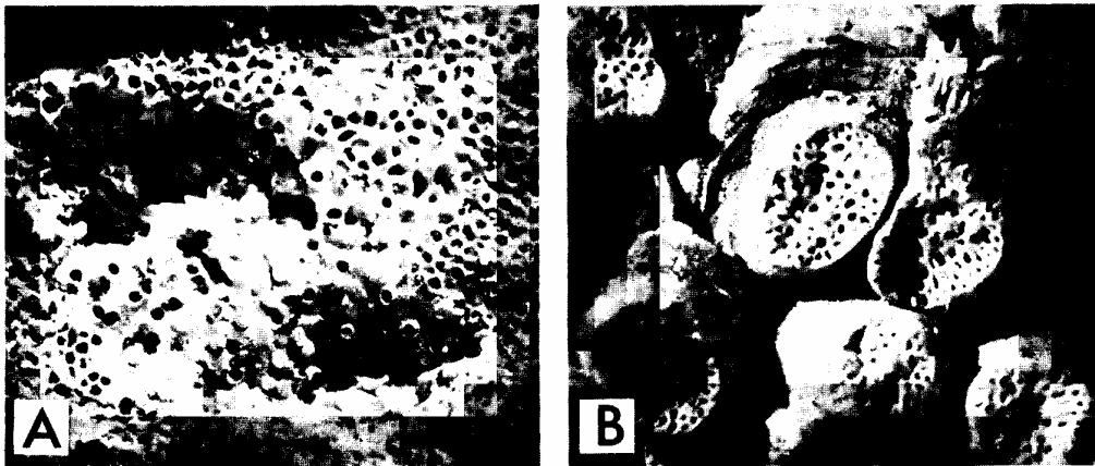
TEXT-FIG. 2. Blumenbachium globosum Koenig. A, surface of a brood chamber pierced by circular autozooecial apertures some of which are occluded, B 1704, Coralline Crag, Sutton, \times 13 . B, cup-shaped subcolonies on the underside of a fractured specimen, D 1495, Coralline Crag, Suffolk, \times 12 .
