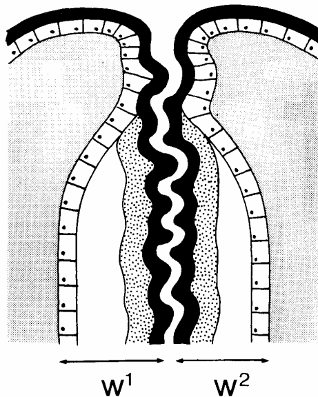
TEXT-FIG. 6. Reconstructed vertical section through the growing edge at the boundary between two contiguous subcolonies of Blumenbachiium globosum Koenig. Inferred exterior walls bounding the two subcolonies are labelled W^1 and W^2 . Each consists of a cuticular layer (solid black), a primary calcified skeletal layer (coarse stipple), a secondary calcified skeletal layer (unshaded), and an epithelial layer (nucleate rectangular cells). Hypostegal coelom is shown by fine stippling. The gap between interdigitating cuticles is exaggerated.
