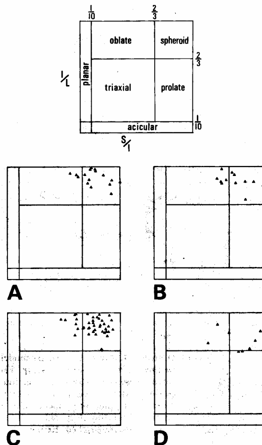
TEXT-FIG. 3. Zingg plots illustrating shape variation among large cyclostome colonies from the Coralline Crag. The upper diagram shows shape nomenclature determined by plotting axial dimension ratios ( S = short axis, I = intermediate axis, L = long axis). A, Meandropora aurantium (Milne Edwards in Lyell), 16 colonies from Aldeburgh. B, Meandropora tubipora (Busk), 12 colonies from Aldeburgh. C, Blumenbachium globosum Koenig, 40 colonies from Aldeburgh and Iken. D, Multifascigera debensis sp. nov., 8 colonies from Ramsholt.
