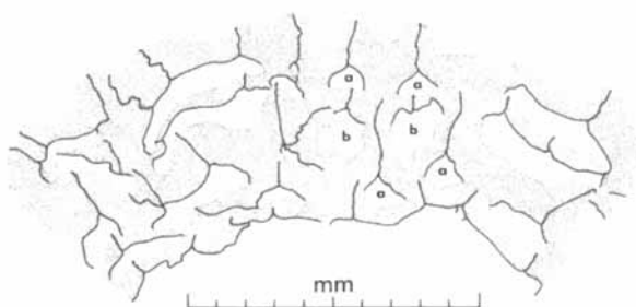
TEXT-FIG. 8. Blumenbachium globosum Koenig, D 6905. Drawing of part of a thin section through a colony showing three or four concentric growth cycles (cf. text-fig. 4b). Dimorphism in the growth cycles is well developed right of centre where two alternating types of lacunae are visible: a, lacunae between low subcolonies; b, lacunae between high ridged subcolonies.
