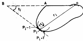
TEXT-FIG. 2. Measurements on a shell outline. The hinge OA is produced to B . P_{i-1} , P_i , P_{i+1} are three consecutive points on the outline. r_c is the radius of curvature, t_i the tangent angle, and r_i the distance from O of point P_i .
