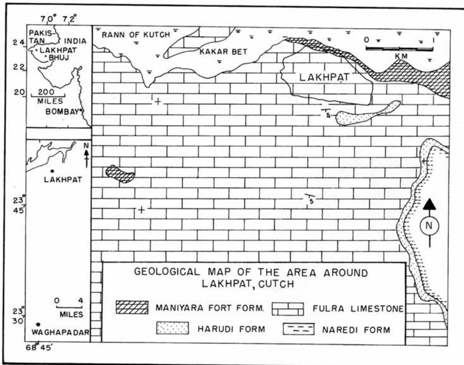
TEXT-FIG. 1. Geological map of the area around Lakhpat, Cutch, western India (modified from Sen Gupta 1964). Inset (upper): Map of a part of western India showing location of Lakhpat. Inset (lower): Map of a part of Cutch showing location of Waghapadar, the type locality of N. obtusus (Sowerby).
