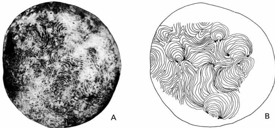
TEXT-FIG. 3. Nummulites obtusus (Sowerby) from the Middle Eocene of Lakhpat, Cutch. 3a, External view of a microspheric specimen. 3b, Drawing showing the complex meandriform septal filaments; CUGD LN 68. Specimen width 16 mm.
