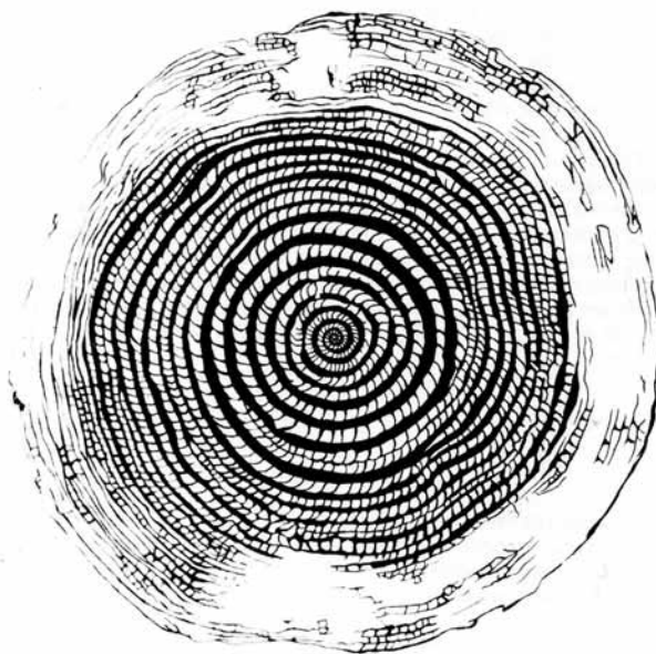
TEXT-FIG. 4. Split equatorial section of a microspheric specimen of Nummulites obtusus (Sowerby), \times 6 ; CUGD LN 85.
