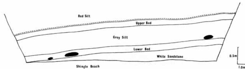
TEXT-FIG. 2. Diagram of the cliff exposure of the Shippard's Chine Pseudofrenelopsis beds. Sides are covered by slumped material from the cliff. Solid black represents fossil logs or rafts of logs.
