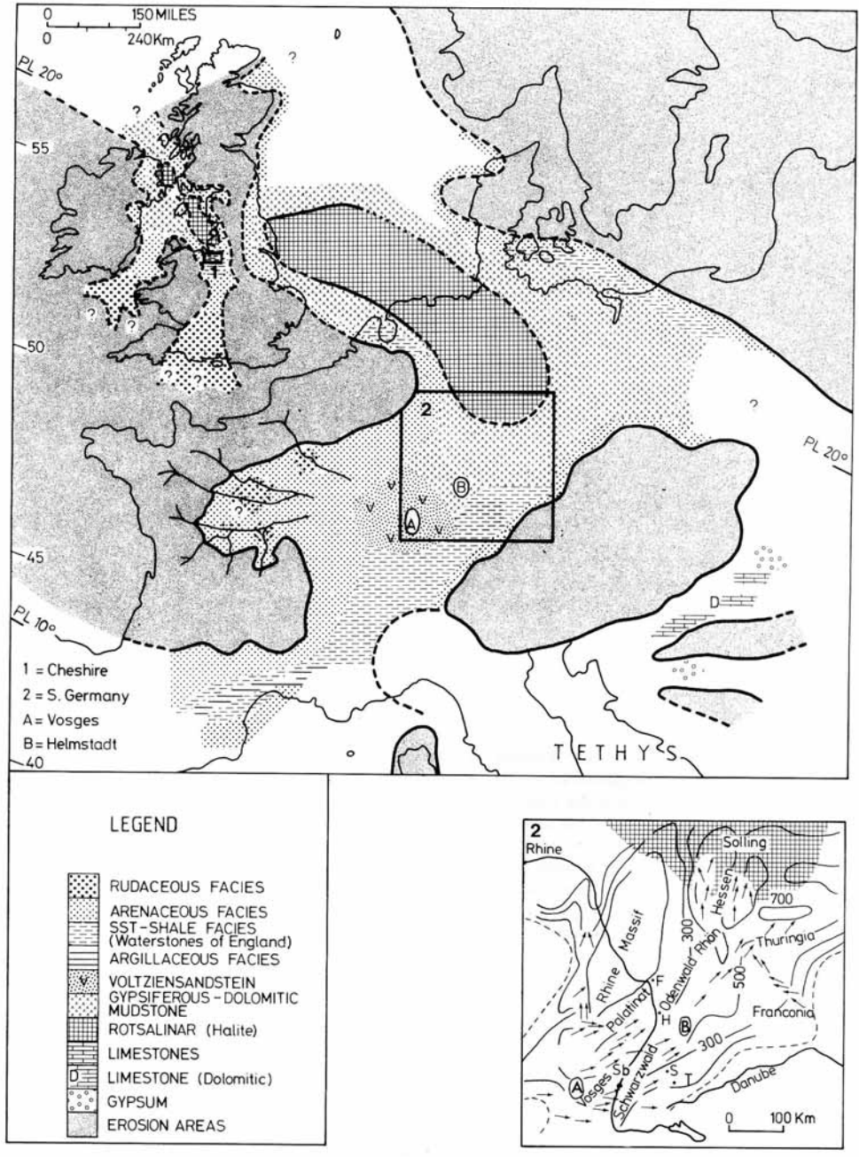
TEXT-FIG. 1. Palaeogeographic map of north-west Europe in Röt times (late Scythian-early Anisian) showing location of areas from which ichnofaunas are compared in this paper. Inset map (2) shows Buntsandstein thickness (in m) and areas of Germany mentioned in text. Abbreviations for place-names as in text-fig. 4. (Data from Warrington 1970b, 1974b; Brennand 1975; Gall et al. 1977).
