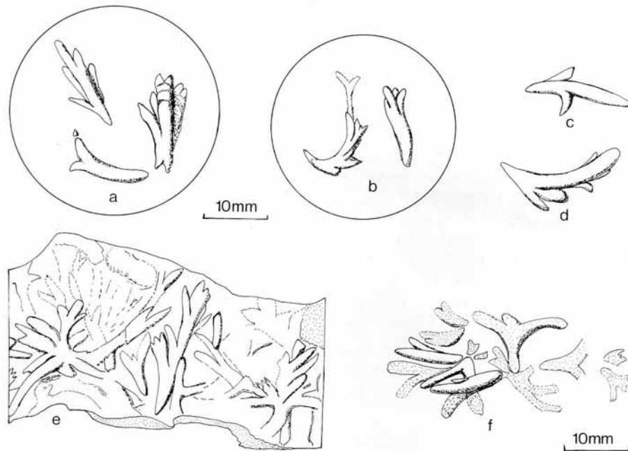
TEXT-FIG. 7. Phycodes curvipalmatum sp. nov. a–e burrows (hypichnia) from holotype slab MGSF 32 (Pl. 89, fig. 2) showing associated (encircled a, b) and isolated, (c, d) recurved and palmate forms, and interwoven burrow network (e); f—paratype MGSF 23 (Pl. 89, fig. 3) (hypichnia) showing radiate 1st order dichotomous branches which overlap and curve upwards.
