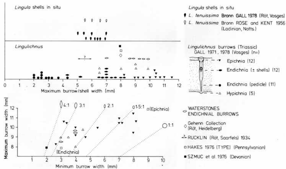
TEXT-FIG. 6. Comparison of width parameters of Lingula shells and Lingulichnus burrows from Triassic sediments of Britain, France, and Germany. Details of Palaeozoic type or syntype specimens of Lingulichnus are also included.
