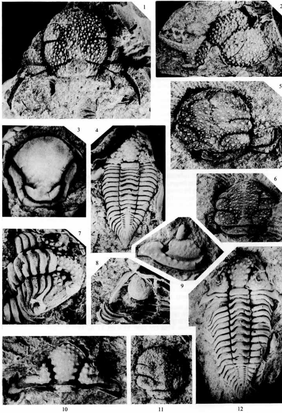
CLARKSON and HOWELLS, Silurian trilobites
