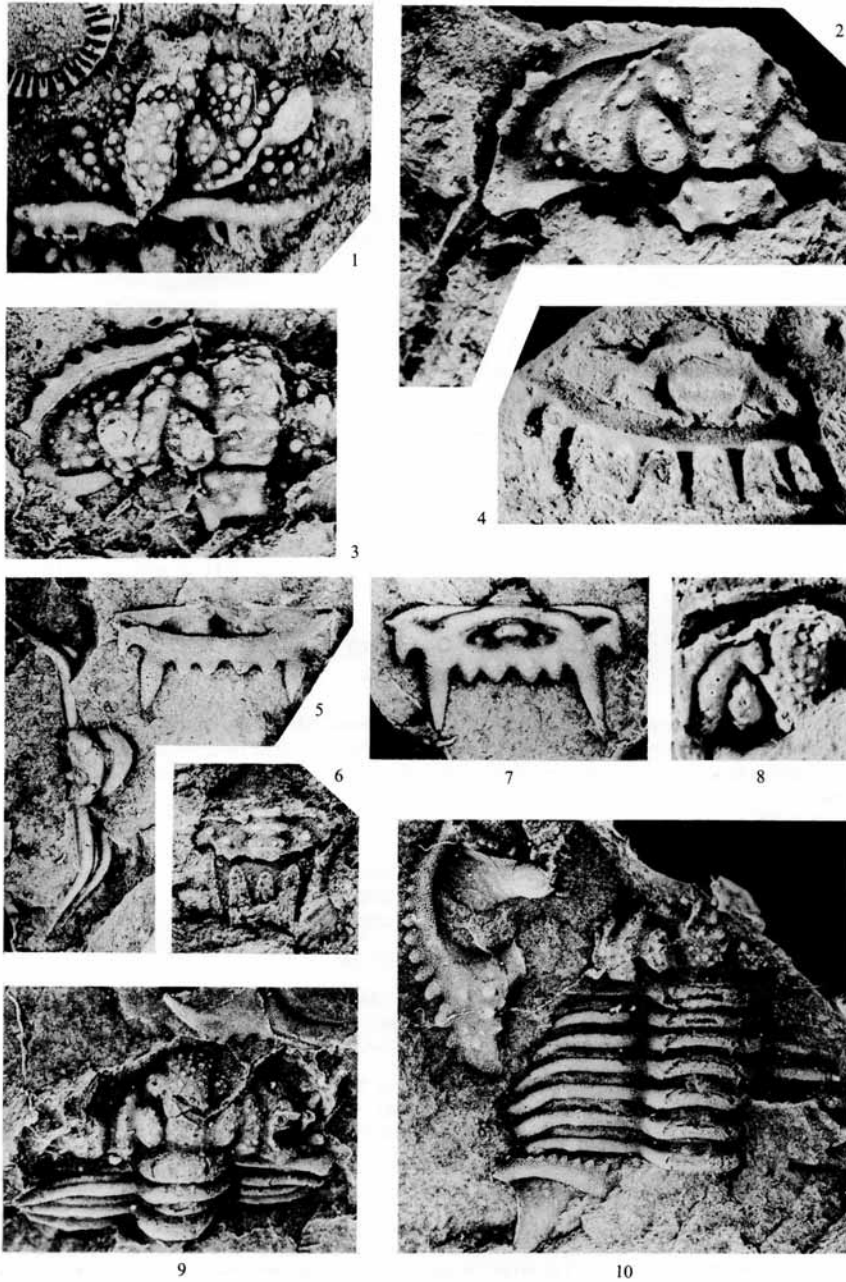
CLARKSON and HOWELLS, Silurian trilobites
