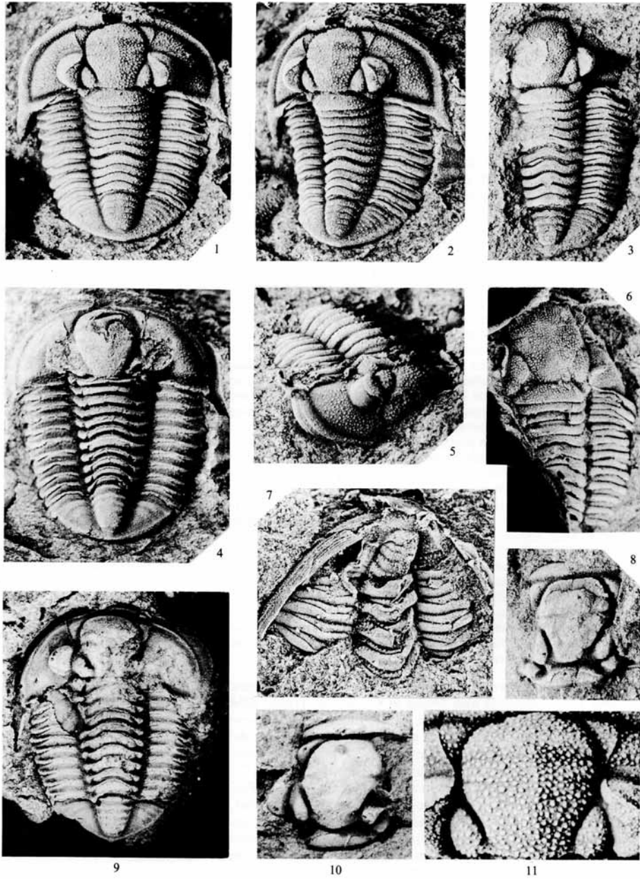
CLARKSON and HOWELLS, Cyphoproetus
