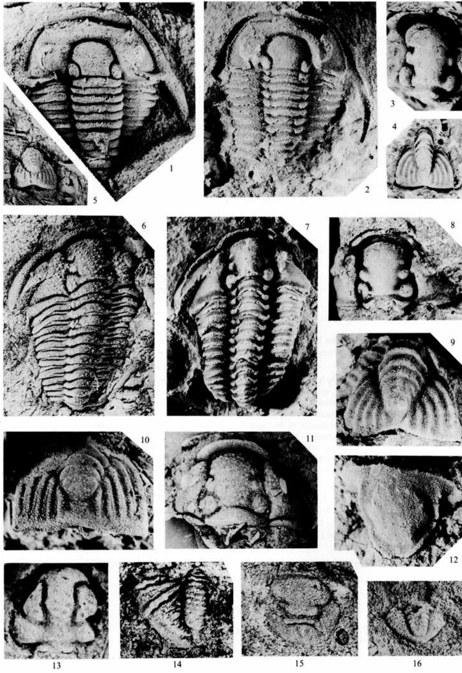
CLARKSON and HOWELLS, Silurian trilobites
