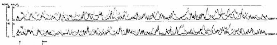
TEXT-FIG. 11. Parallel electron microprobe traverses across Hearne Formation stromatolite lamination (GSM 77325) recording the elements Si and Al. The traverses employed a line probe of dimensions 200 \times 40 \mu\text{m} oriented parallel to the lamination,
