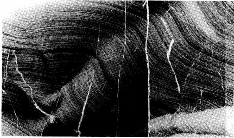
TEXT-FIG. 7. Thin section of Hearne Formation stromatolite (GSM 77323) showing a very uniform development of micritic lamination, \times 1.6 .
