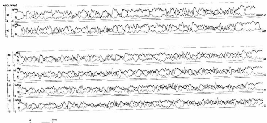
TEXT-FIG. 10. Parallel electron microprobe traverses across Hearne Formation stromatolite lamination (GSI 77325) recording elements Si and Mg. Traverses G28BP-I to IV employed a 200 \times 40\ \mu\text{m} line probe and 200\ \mu\text{m} apart from each other. Traverses V and VI employed a 40\ \mu\text{m} diameter probe, and V was positioned between I and II, while VI was 300\ \mu\text{m} away on the other side of traverse I.
