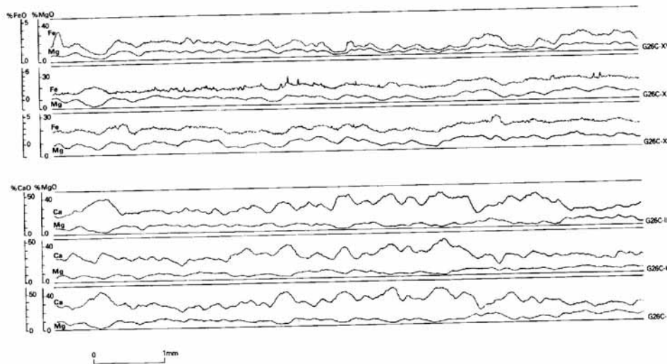
TEXT-FIG. 9. Parallel electron microprobe traverses across Hearne Formation stromatolite lamination (GSI 77322), recording the elements Fe and Mg, and Ca and Mg. The traverses within each set of three are about 500\ \mu\text{m} apart and employed a line probe of dimension 400 \times 150\ \mu\text{m} oriented parallel to the lamination.
