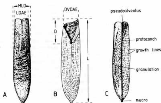
TEXT-FIG. 2. Diagram showing the morphological elements of the Gonoteuthis guard. A, ventral view. B, left lateral view of a ground guard. C, cut-away dorsal view. MLD = maximum lateral diameter; LDAE = lateral diameter at the alveolar end; D = depth of the pseudoalveolus; L = length of guard; DVDAE = dorso-ventral diameter at the alveolar end.
