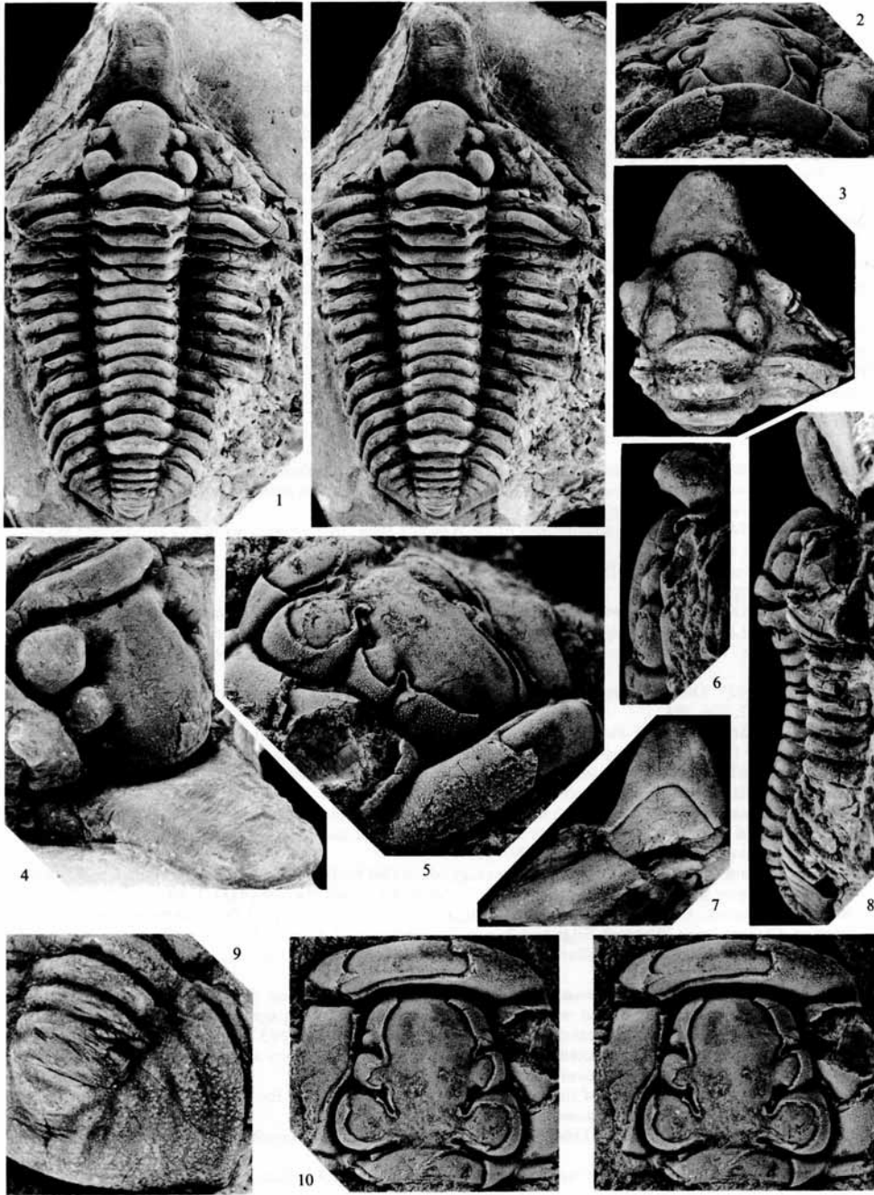
SIVETER, Calymenid trilobites
