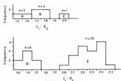
TEXT-FIG. 1. Histogram of ratio of width between palpebral lobes to width of glabella at lobe 2p (= variates J_1 and K_2 of Siveter 1977, p. 338, fig. 1). A. Spathacalymene nasuta . B. Diacalymene diademata . C. ' Calymene ' allportiana . D. Calymene blumenbachii . E. Tapinocalymene : T. volsoriforma , n=6; T. vulpecula , n=4; T. nodulosa , n=10.
