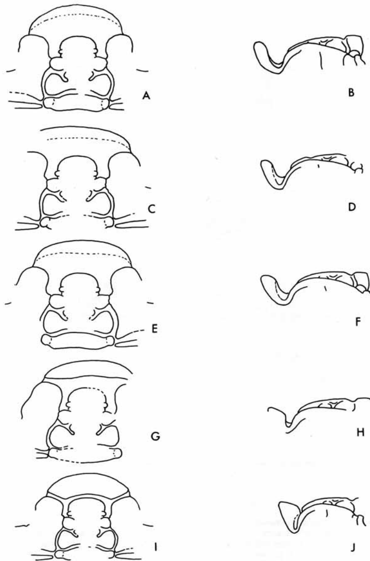
TEXT-FIG. 2. Proposed evolutionary lineage in Tapinocalymene gen. nov. Dorsal and lateral outlines of cranidia, all \times 2 . A, B. T. nodulosa , HM A212/1, pl. 97, figs. 1, 11. C, D. T. nodulosa , GSM Zs183, pl. 98, figs. 10, 11. E, F. T. nodulosa GSM Zs195, pl. 98, figs. 6, 12. G, H. T. vulpecula , holotype, NMW 77.31G.1, pl. 100, figs. 1, 2. I, J. T. volsoriforma , holotype, GSM Zs63, pl. 99, figs. 1, 2.
